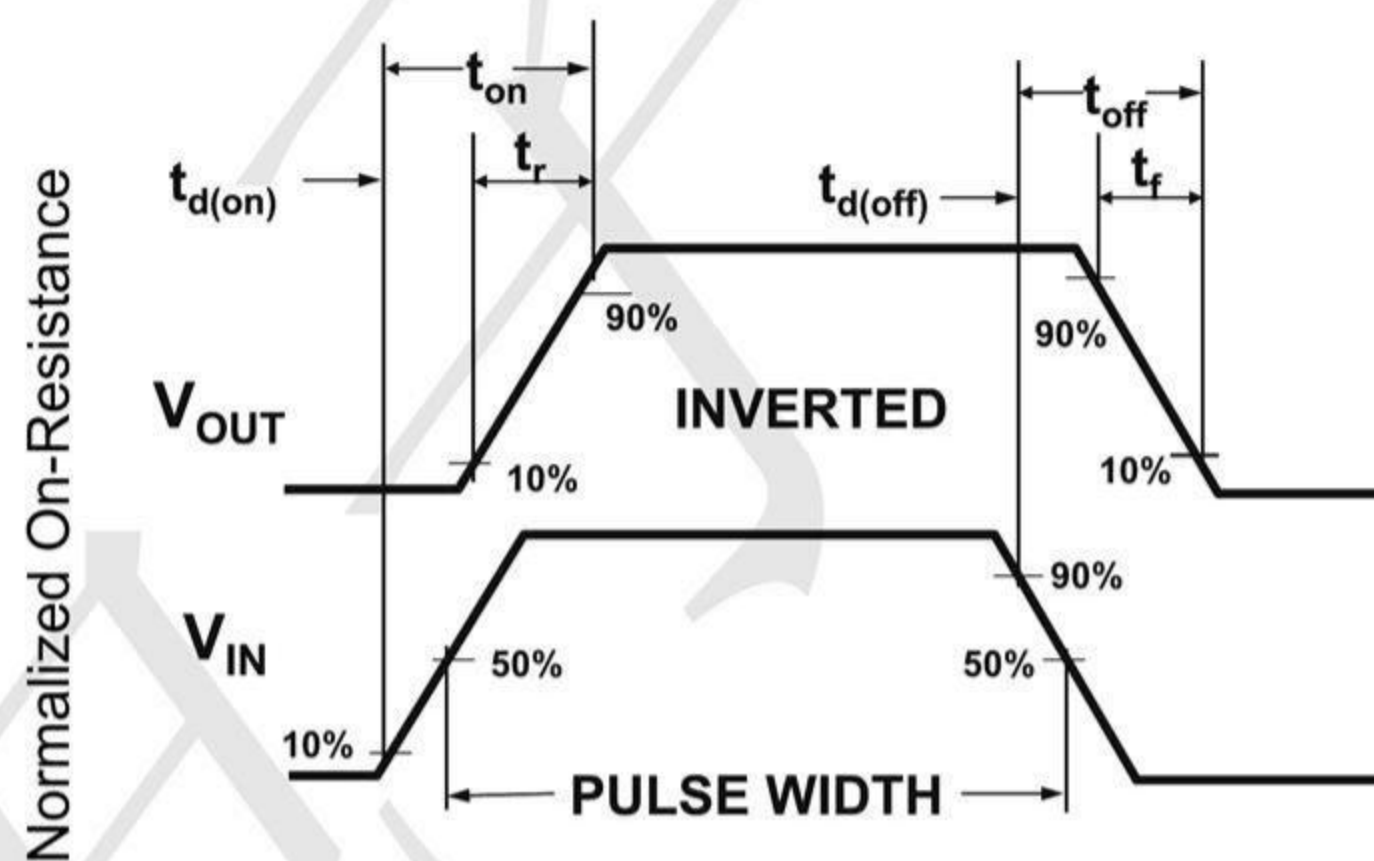
Figure 2: Switching Waveforms
