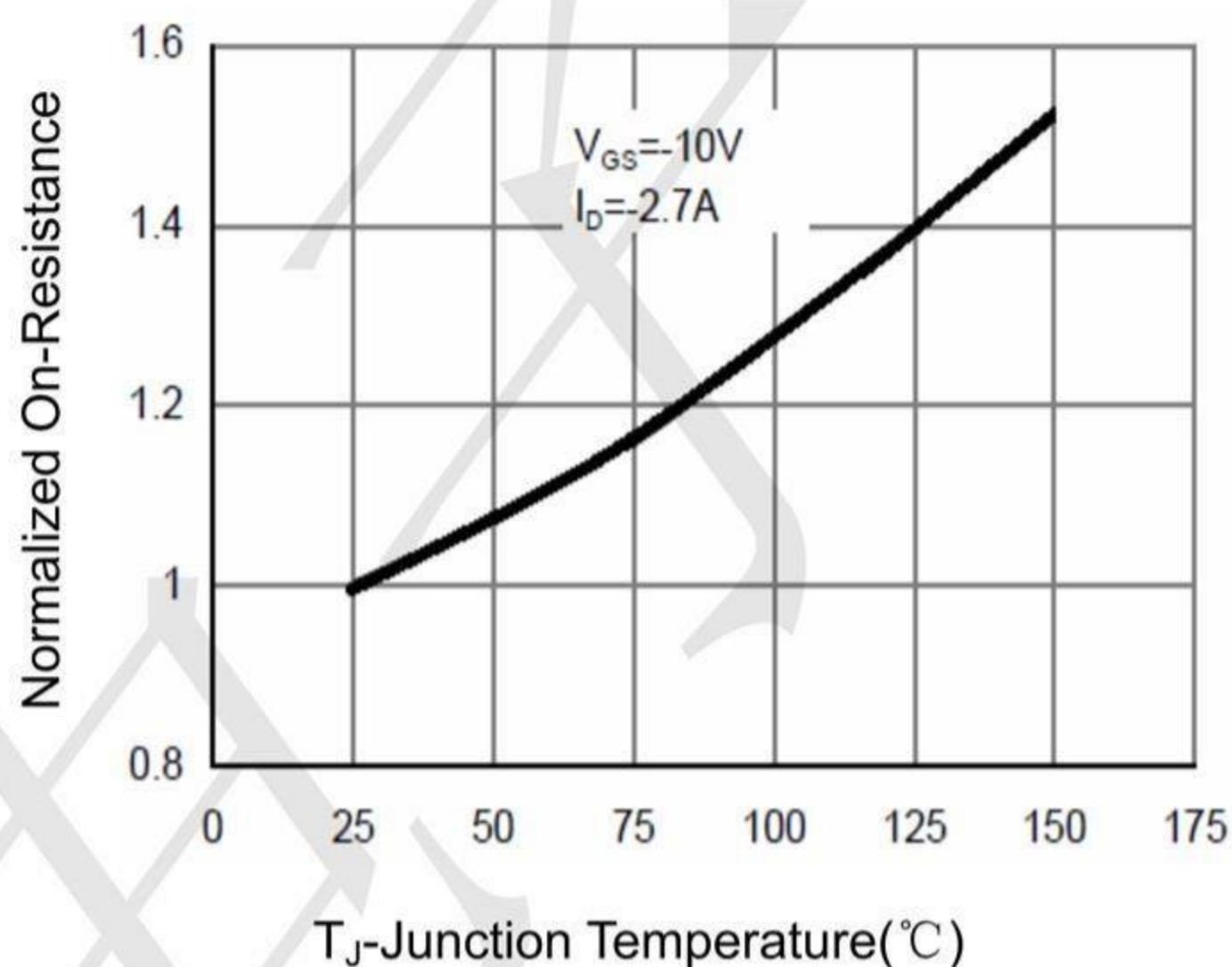
Figure 8 Drain-Source On-Resistance
