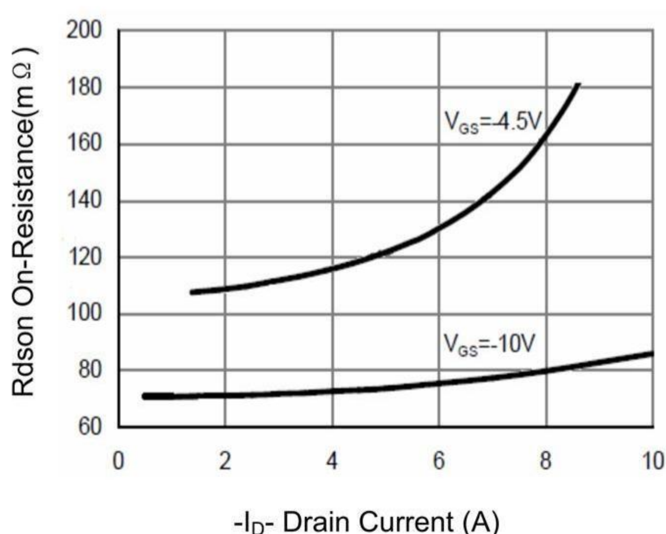
Figure 6 Drain-Source On-Resistance
