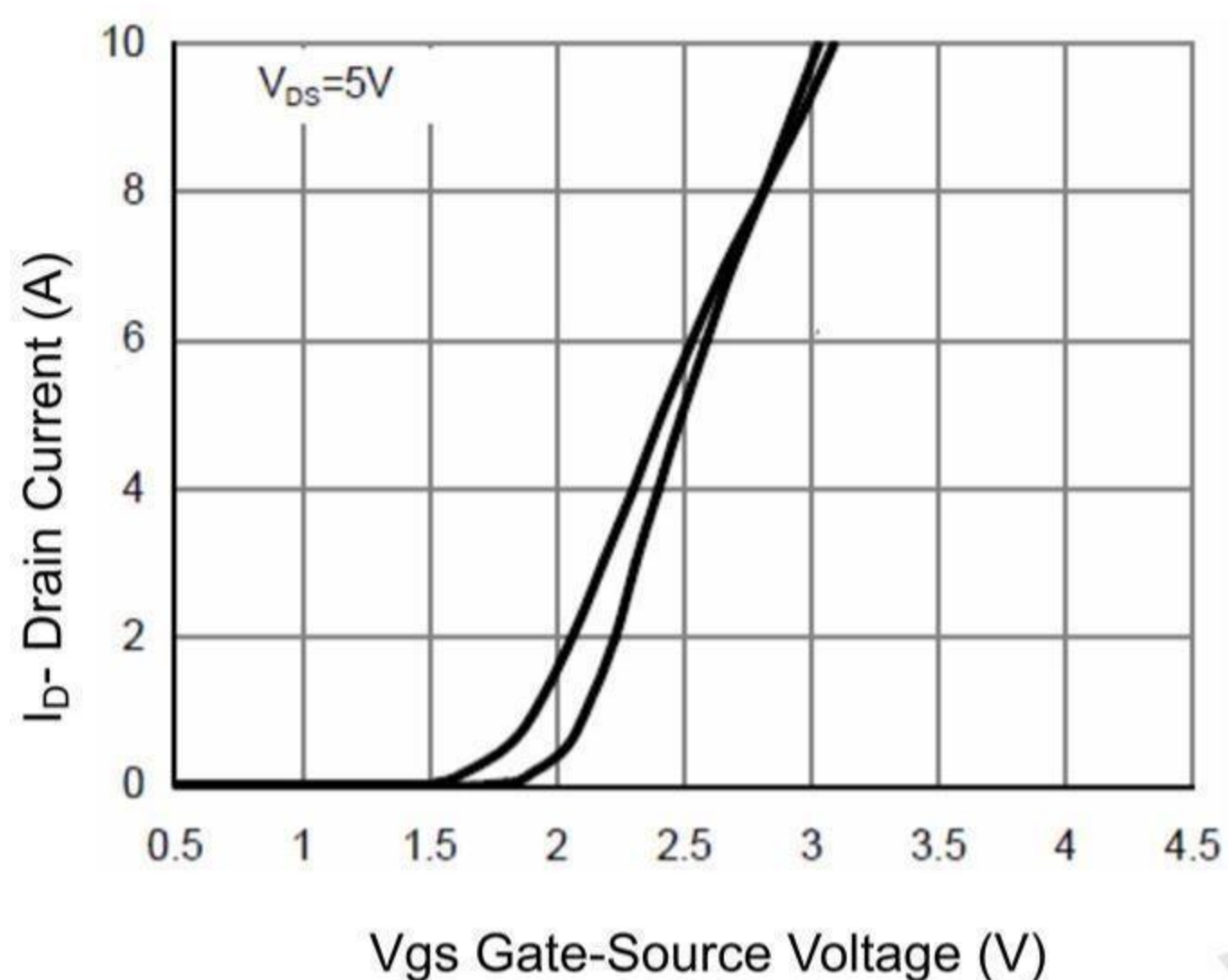
Figure 7 Transfer Characteristics
