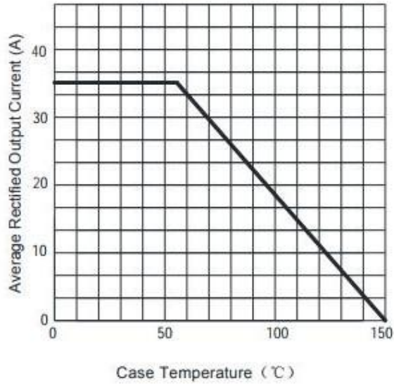
FIG1:Io-Tc Curve
