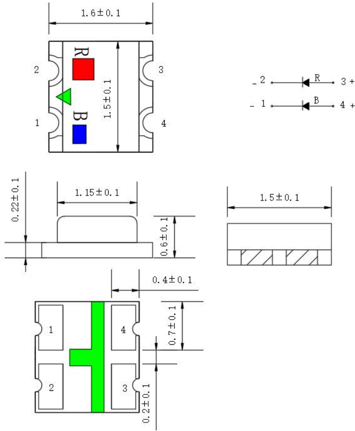
Recommended Solder Pad Design 推荐焊盘设计
