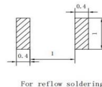
Recommended Solder Pad Design 推荐焊盘设计
