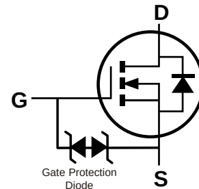
Equivalent Circuit
