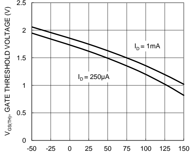
T_J , JUNCTION TEMPERATURE ( ^{\circ}C ) Figure 8. Gate Threshold Variation vs. Junction Temperature
