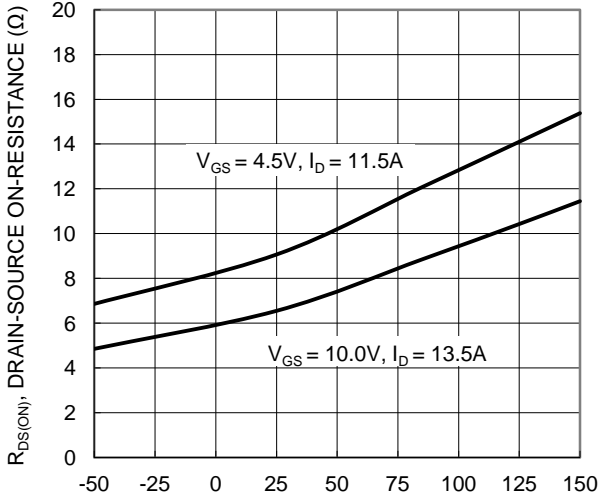
T_J , JUNCTION TEMPERATURE ( ^{\circ}C ) Figure 7. On-Resistance Variation with Temperature
