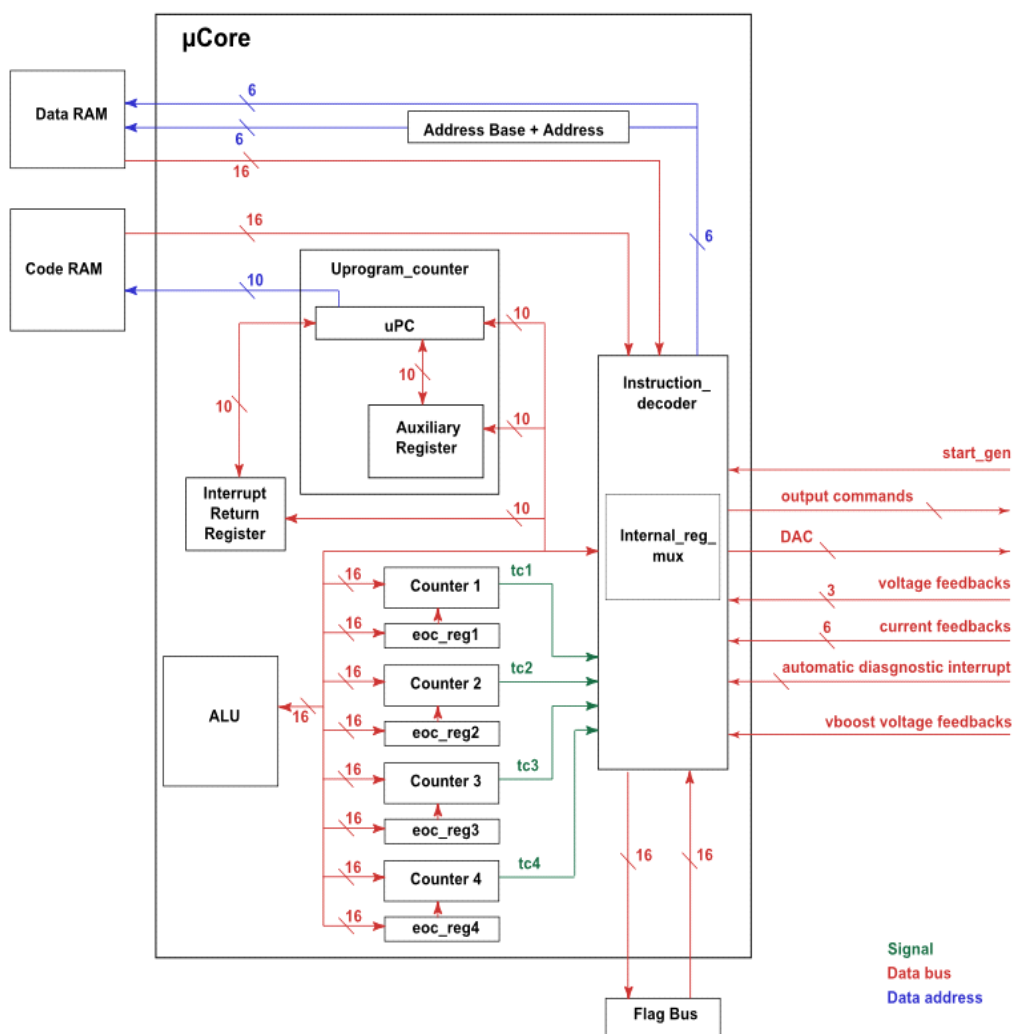
Figure 36. Microcore block diagram
