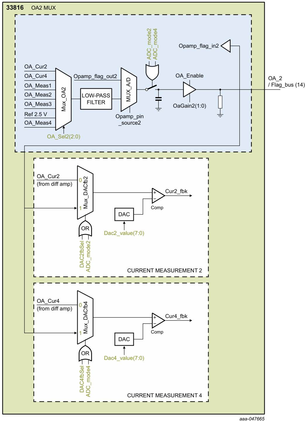
Figure 23. Measurement function OA2 detail
