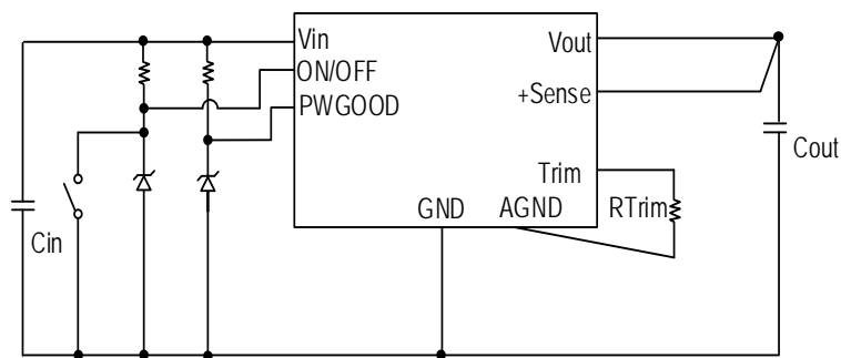
MYMGM1R816ELA5RA Cin: 22uF/25V x 2pcs Co: 220uF/4V x 3pcs
