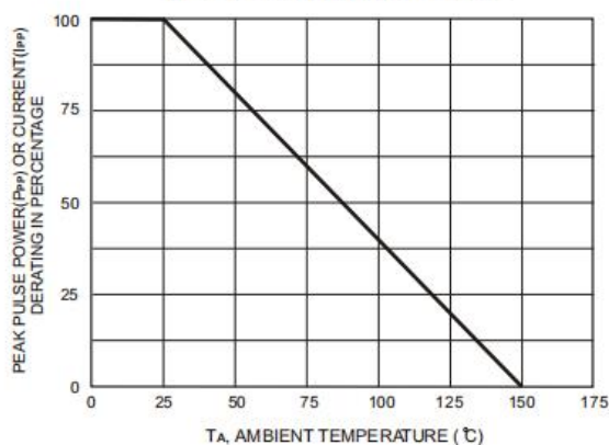
FIG.2-PULSE DERATING CURVE
