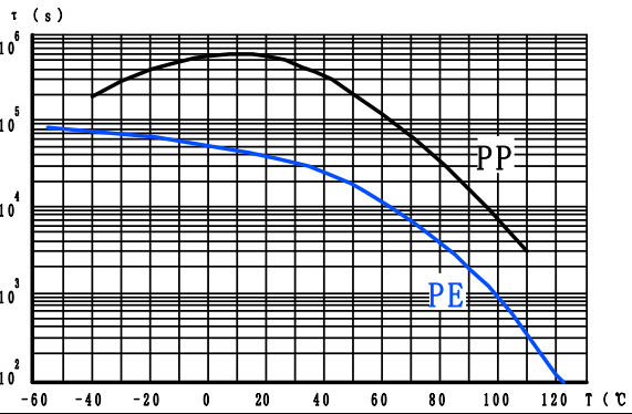
绝缘电阻与温度的关系(CR value) IR vs. Temperature
