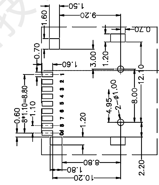
RECOMMENDED P.C.B HOLE LAYOUT COMPONENT SIDE VIEW(TOLERANCE: +/-0.05)
