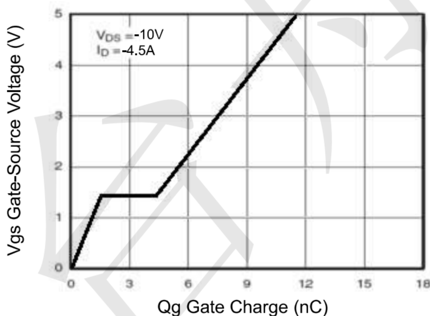
Figure 11 Gate Charge
