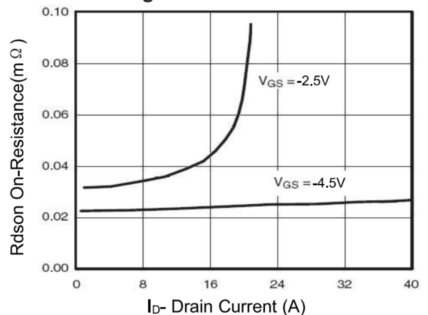
Figure 6 Drain-Source On-Resistance
