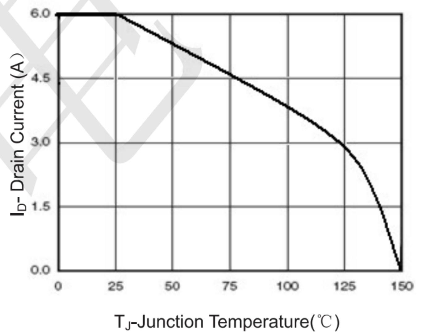
Figure 4 Drain Current
