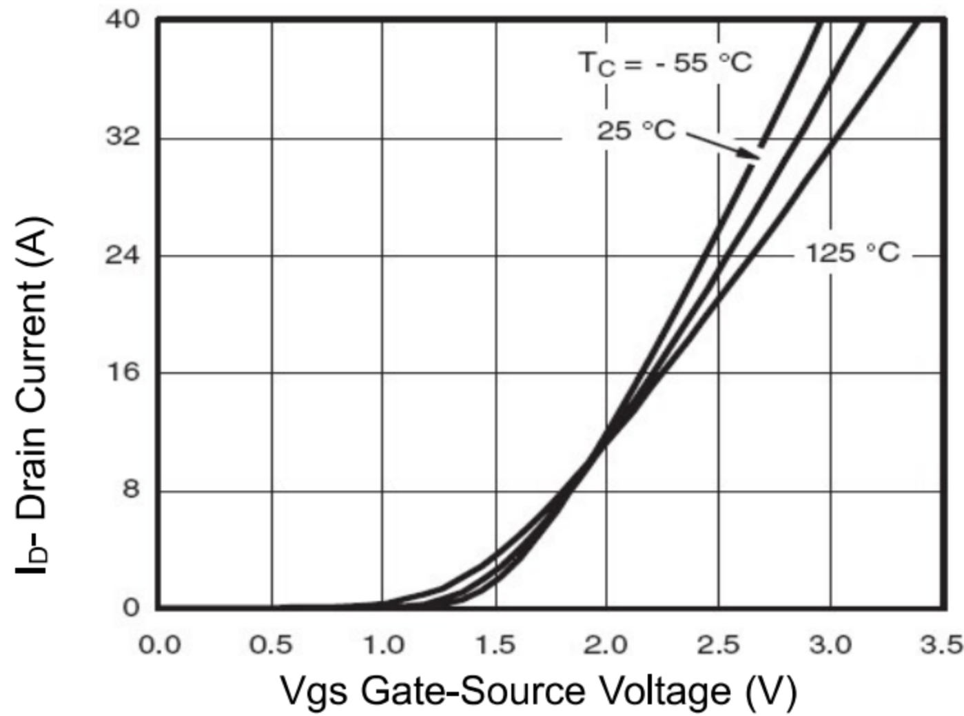
Figure 7 Transfer Characteristics
