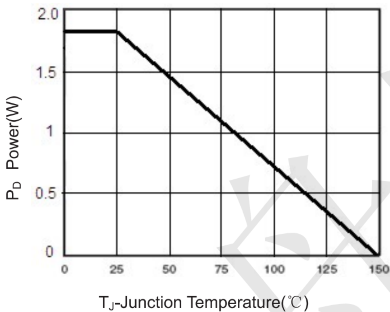
Figure 3 Power Dissipation
