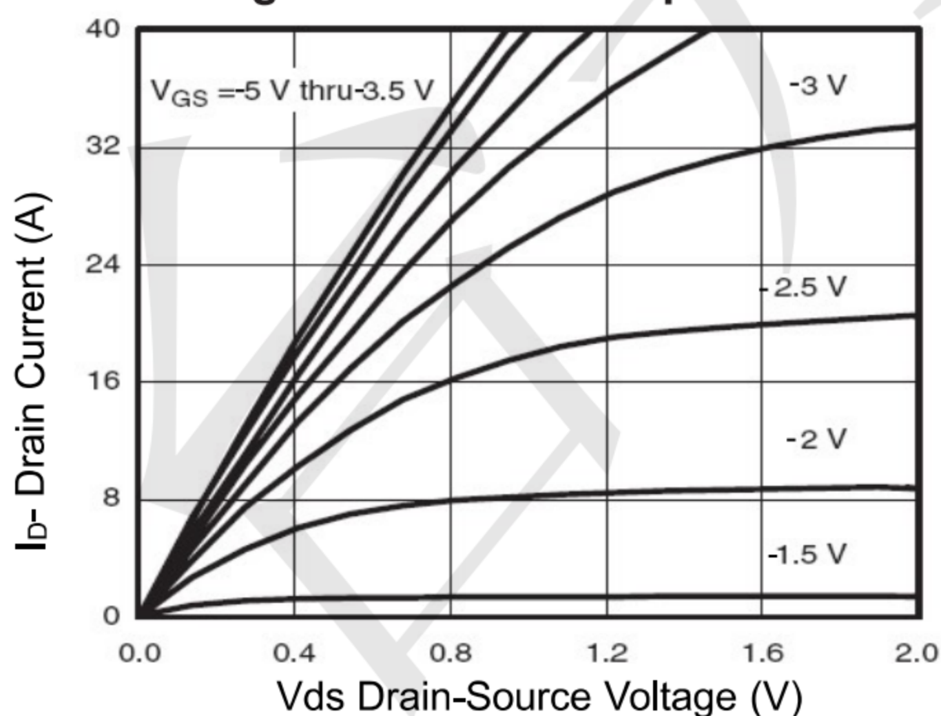
Figure 5 Output Characteristics
