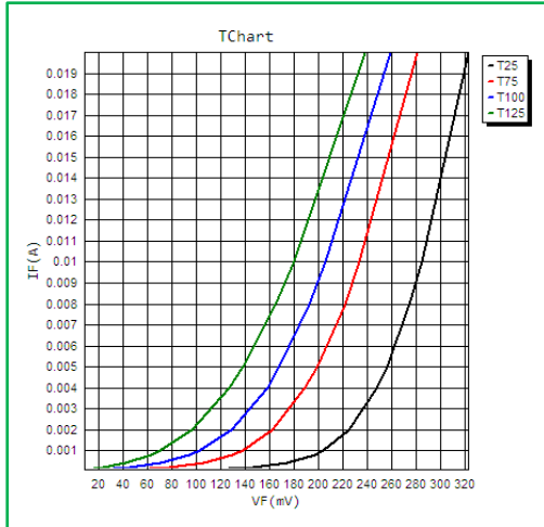
Forward Characteristics
