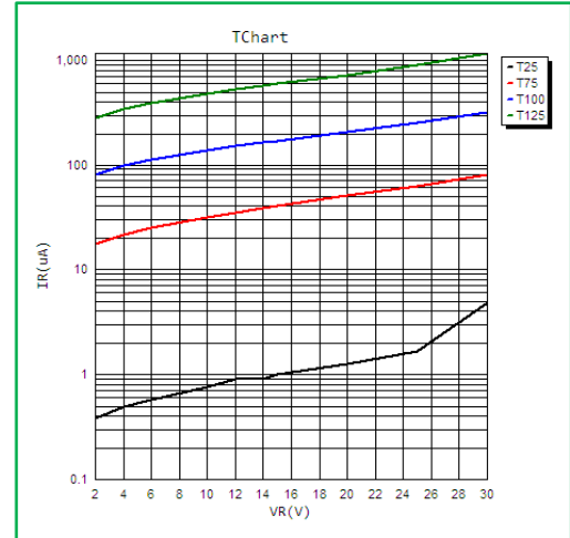
Reverse Characteristics
