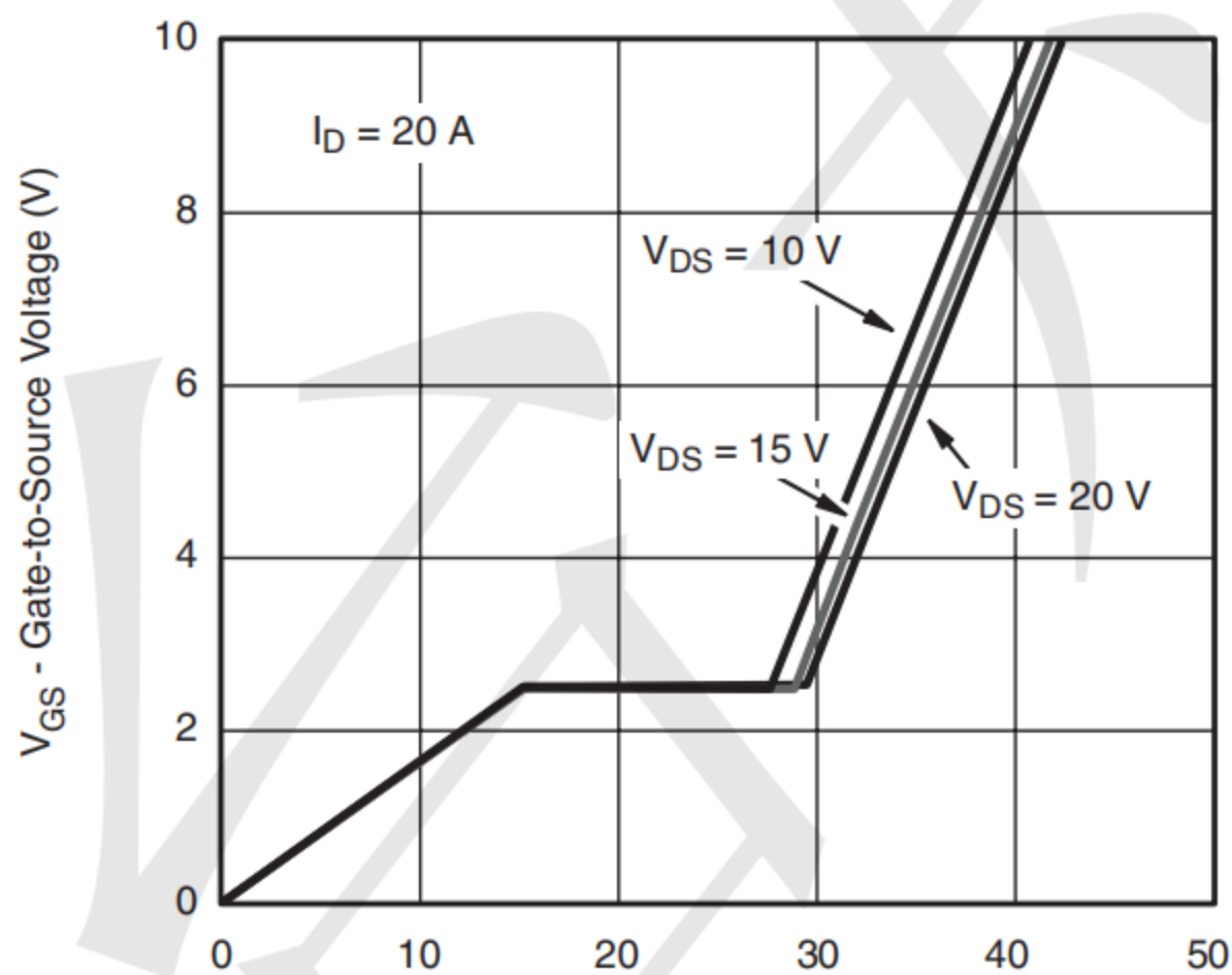
Gate Charge
