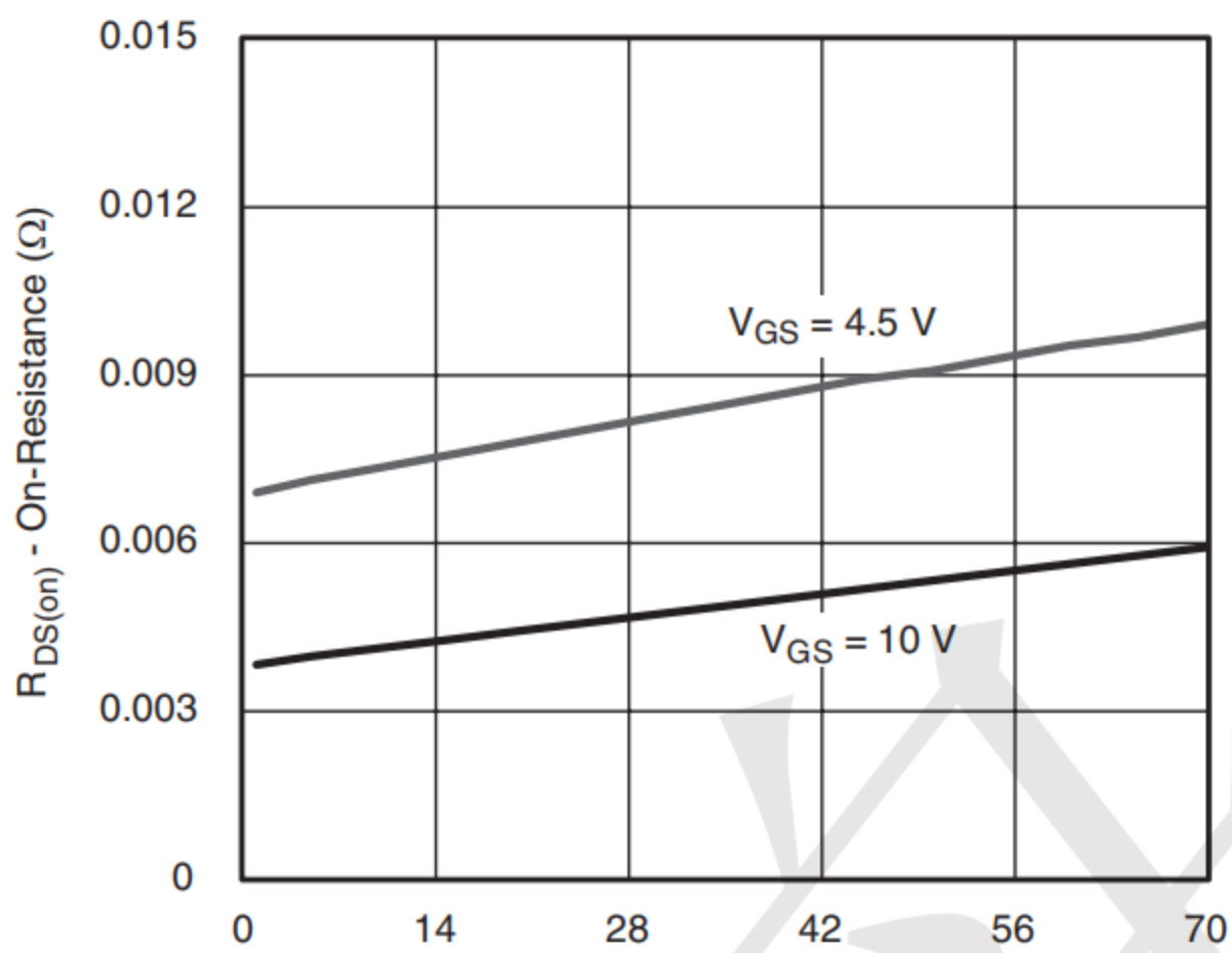
On-Resistance vs. Drain Current
