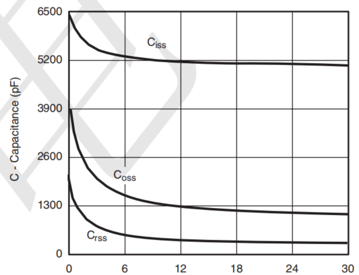
Capacitance
