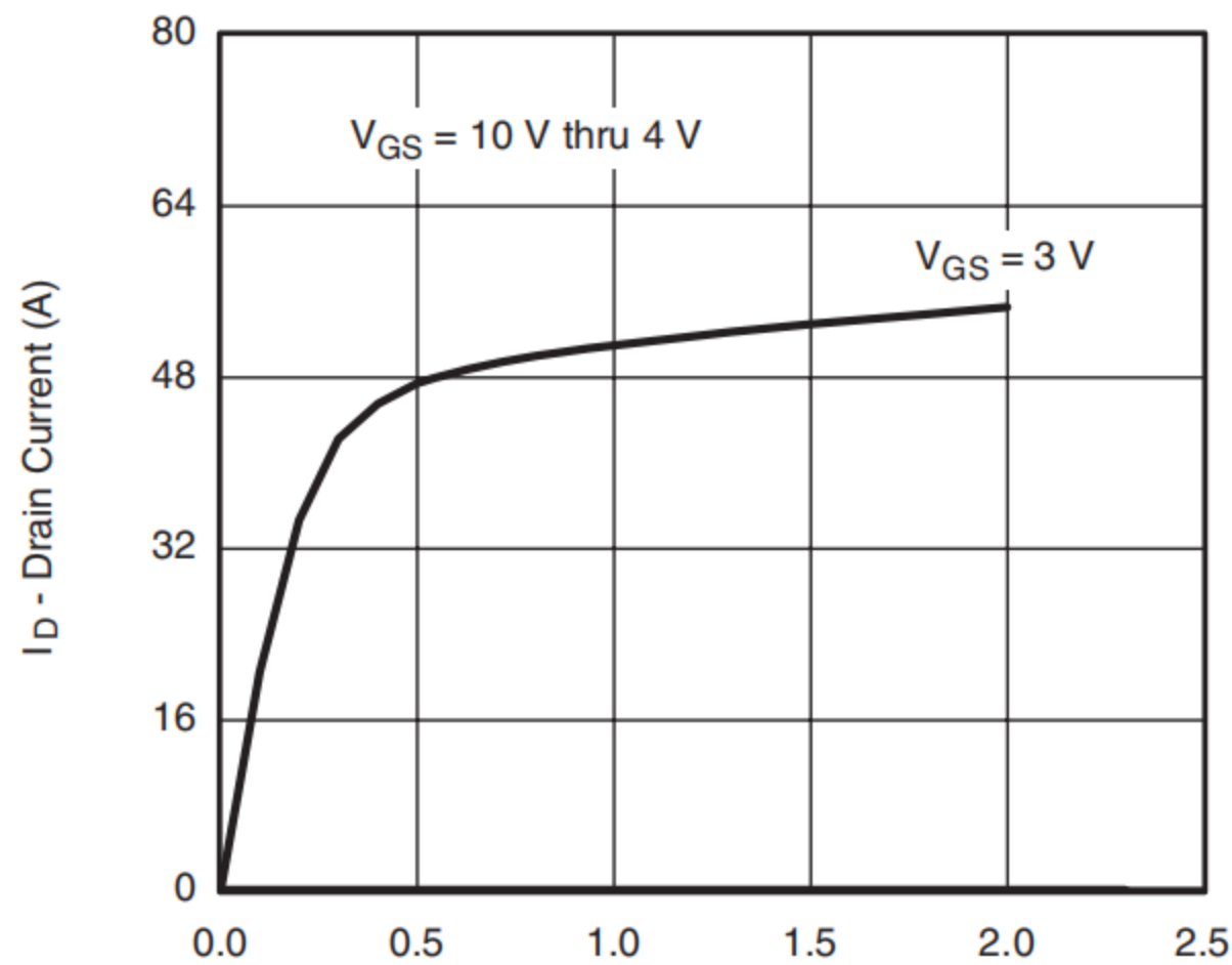
Output Characteristics
