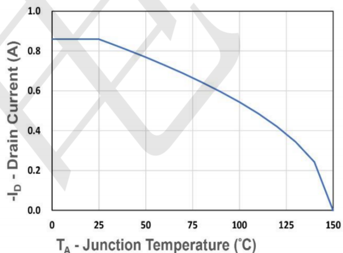
Figure 10. Drain Current
