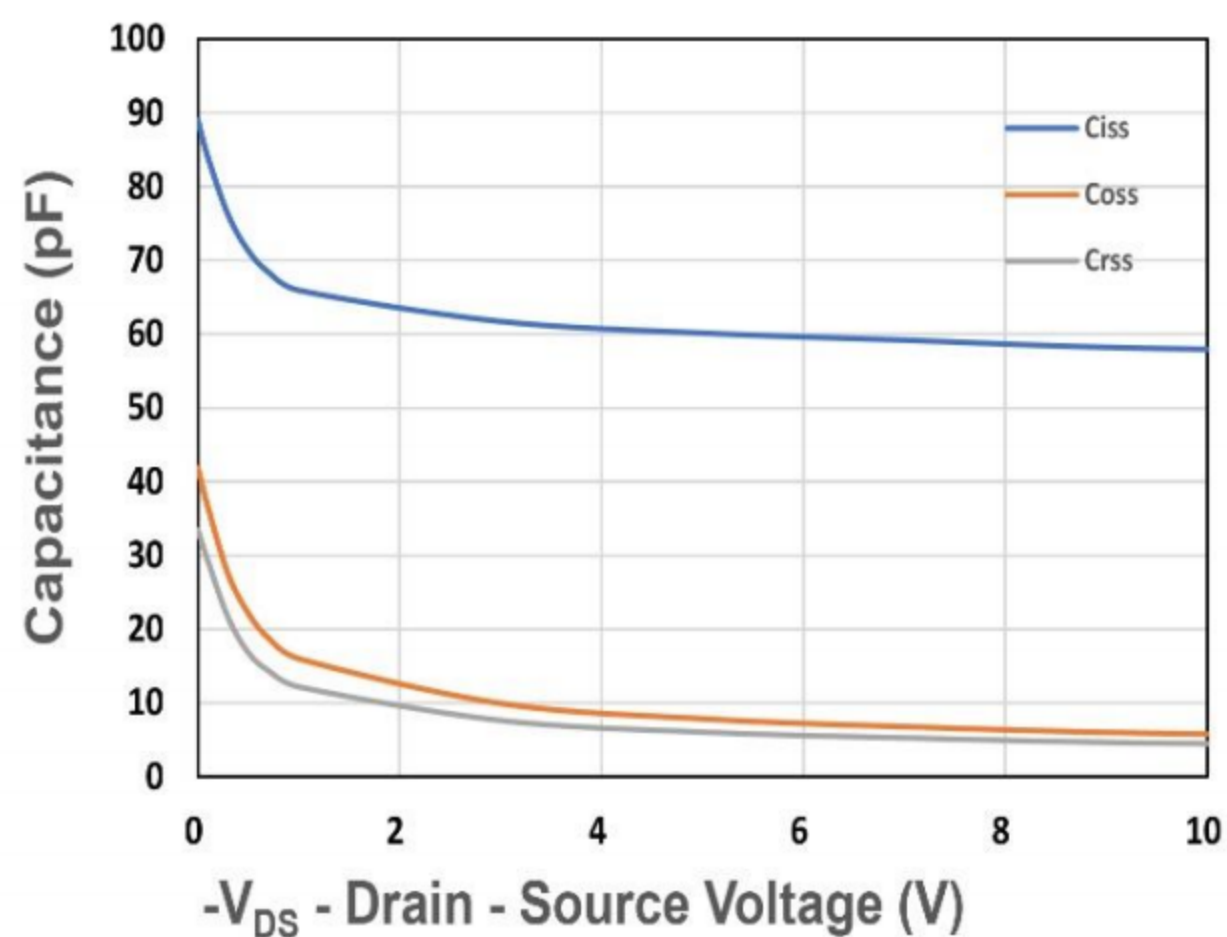
Figure 7. Capacitance
