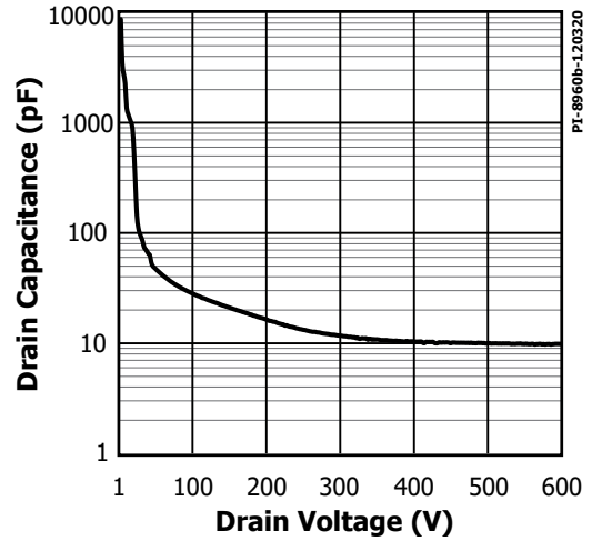
Figure 28. C_{oss} vs. Drain Voltage (INN3996CQ).
