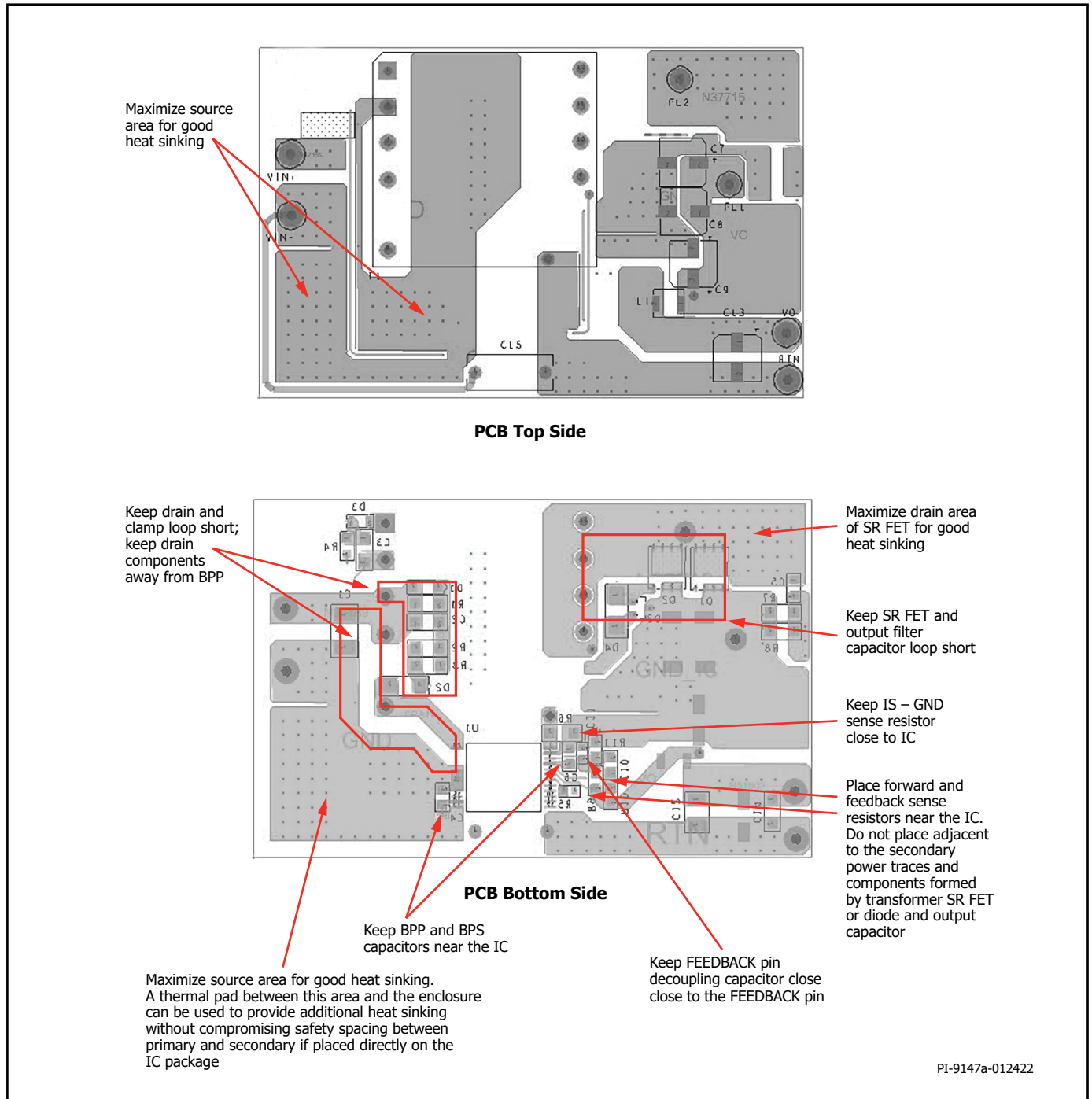
Figure 15. PCB Design.
