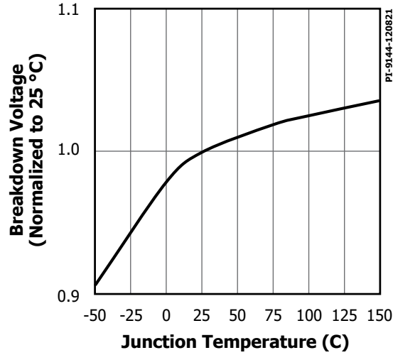
Figure 25. Breakdown Voltage vs. Temperature (INN3977CQ).
