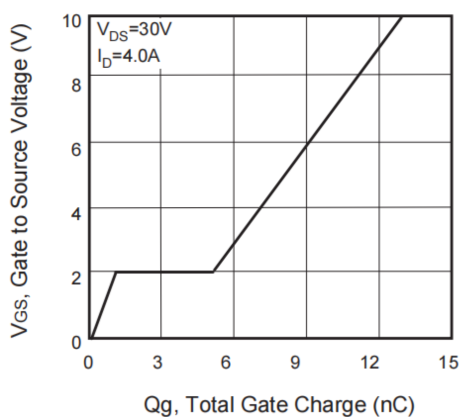
Figure 7. Gate Charge
