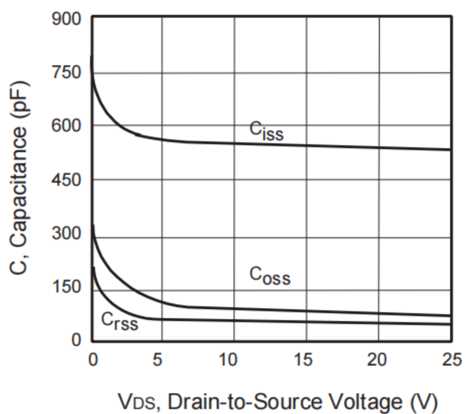
Figure 3. Capacitance
