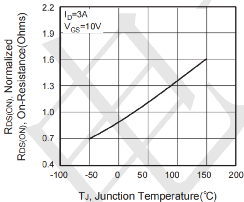
Figure 4. On-Resistance Variation with Temperature
