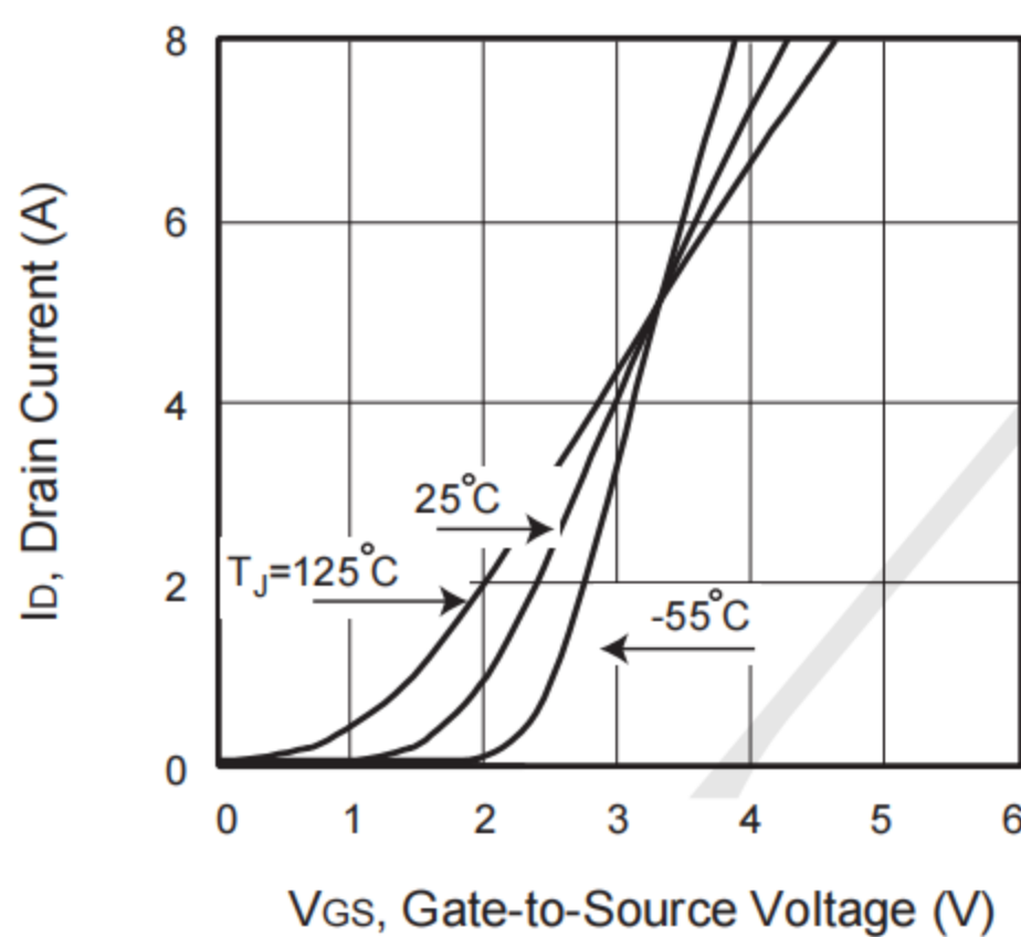
Figure 2. Transfer Characteristics
