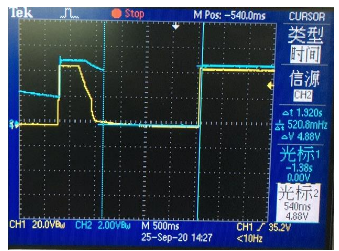
Output response & load (5.5V / 5A)
