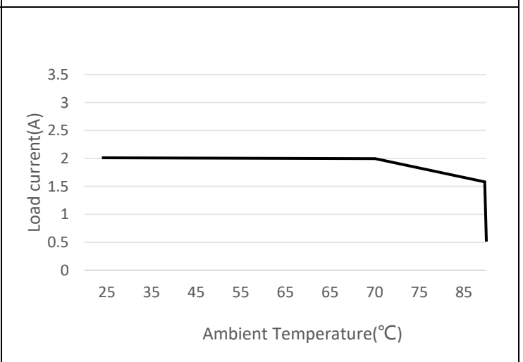
Derating
