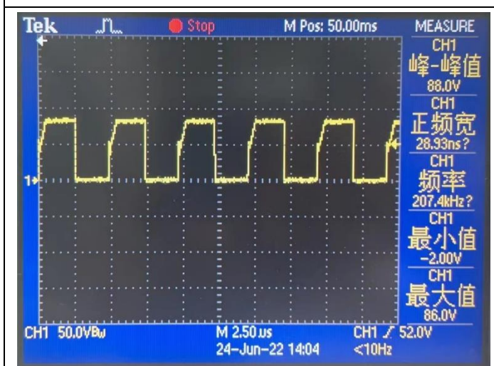
Transformer Switch Waveform
