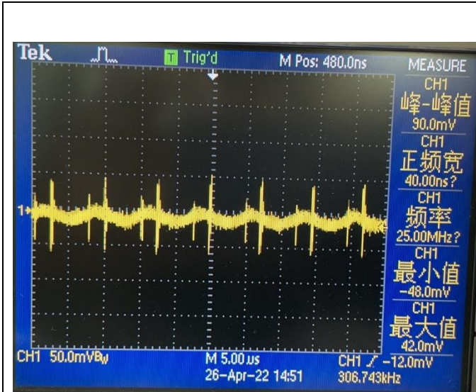
Noise (VIN = 48V, IO = 2A, 5 ~ 20MHz bandwidth)
