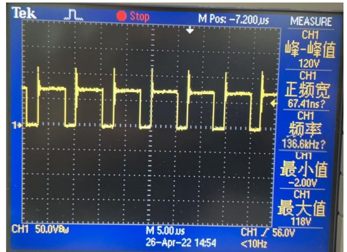
PoE switching waveform
