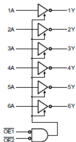
Figure 1. Logic symbol
