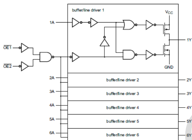
Figure 4. Logic diagram
