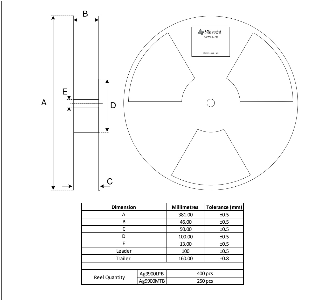
Figure 26: Reel Dimensions
