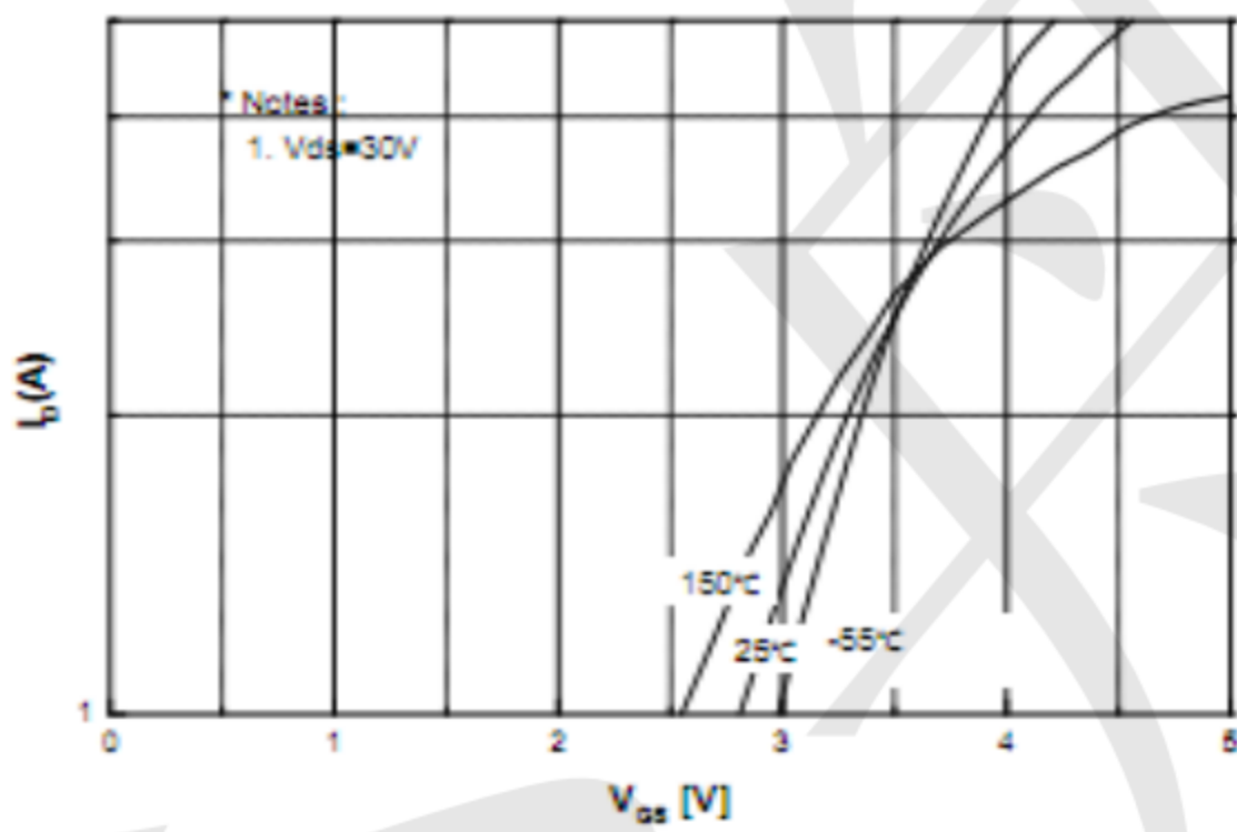
Fig.5 Transfer Characteristics
