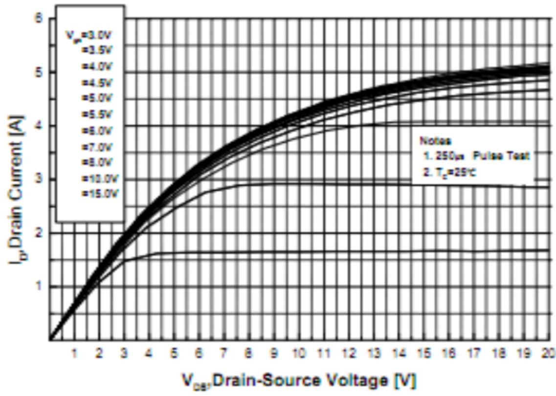
Fig.1 On-Region Characteristics
