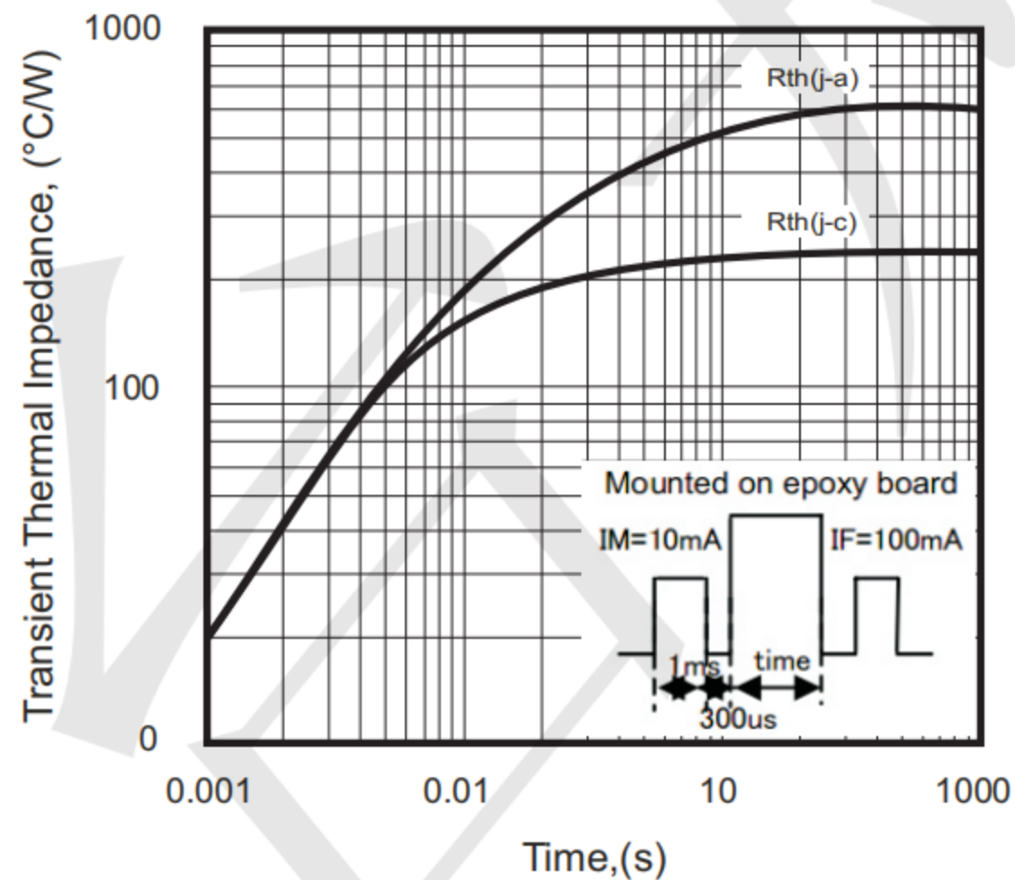
Fig.5 - Rth-t Characteristics
