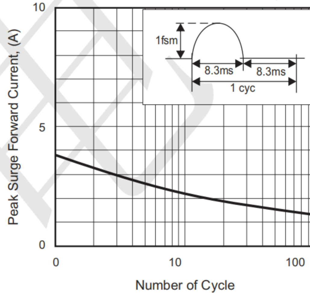
Fig.4 - IFSM-Cycle Characteristics
