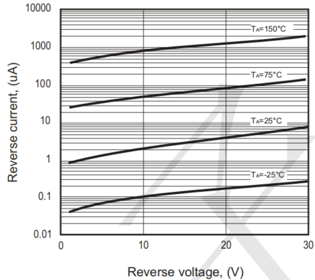
Fig.2 - Reverse Characteristics
