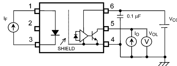
Fig. 13.1.2 V_{OL} Test Circuit
