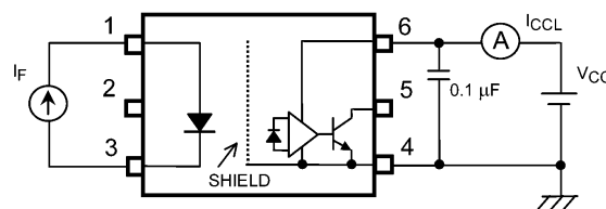
Fig. 13.1.4 I_{CCL} Test Circuit
