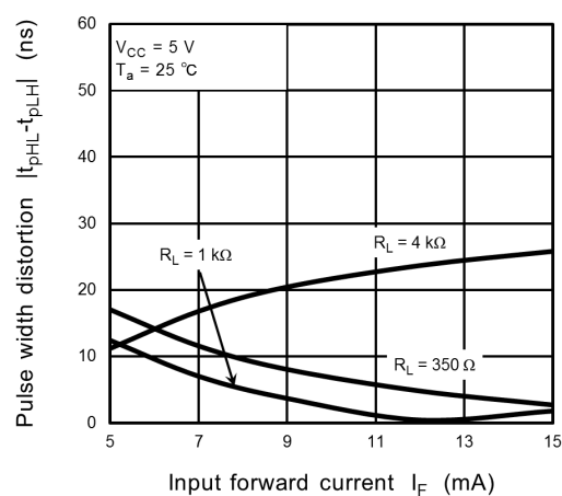
Fig. 13.2.16 |t_{pHL} - t_{pLH}| - I_F
