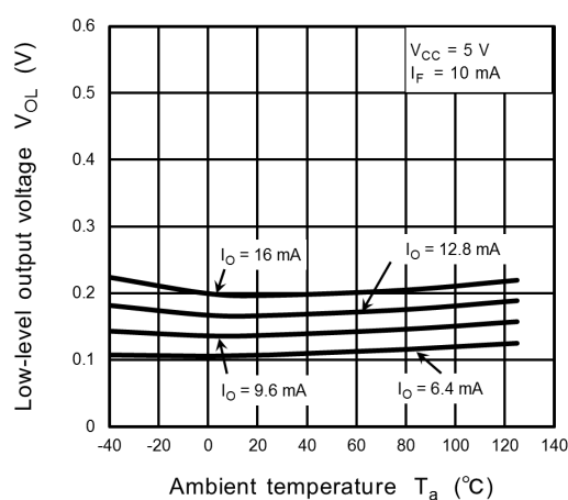
Fig. 13.2.3 V_{OL} - T_a
