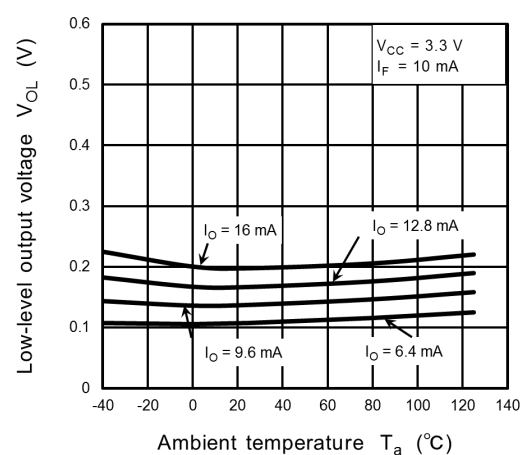
Fig. 13.2.4 V_{OL} - T_a
