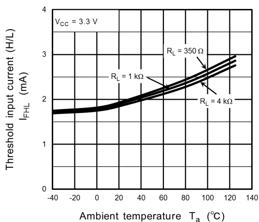
Fig. 13.2.8 I_{FHL} - T_a
