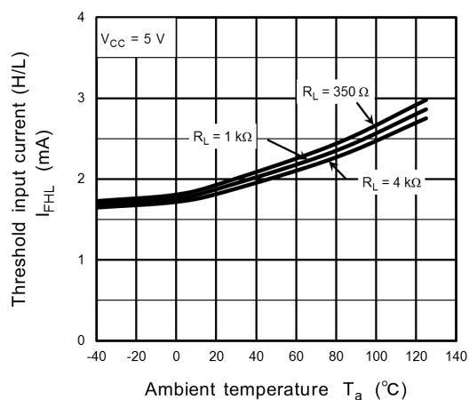
Fig. 13.2.7 I_{FHL} - T_a
