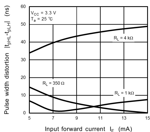
Fig. 13.2.18 |t_{pHL} - t_{pLH}| - I_F
