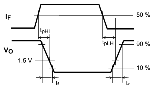
Fig. 13.1.5 Switching Time Test Circuit and Waveform
