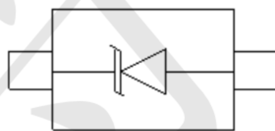
SOD-523 (Top View)
