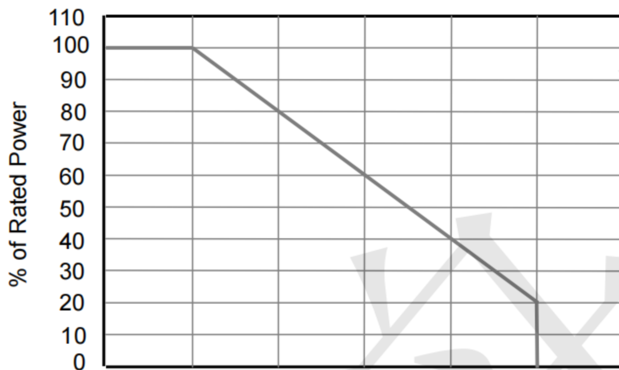
Fig3. Power Derating Curve
