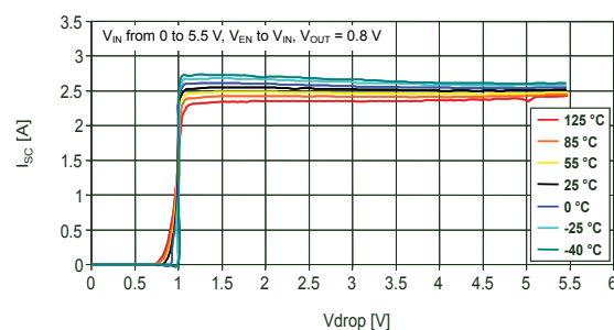
Figure 9. Short-circuit current vs. drop voltage
