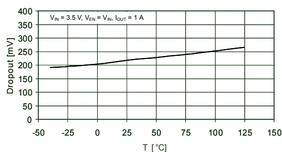
Figure 7. Dropout voltage vs. temperature ( V_{OUT} = 1.5 V )
