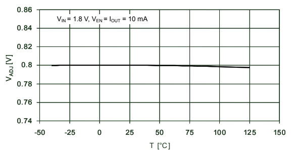
Figure 4. V_{ADJ} accuracy
