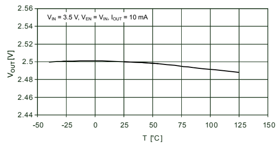
Figure 5. V_{OUT} accuracy
