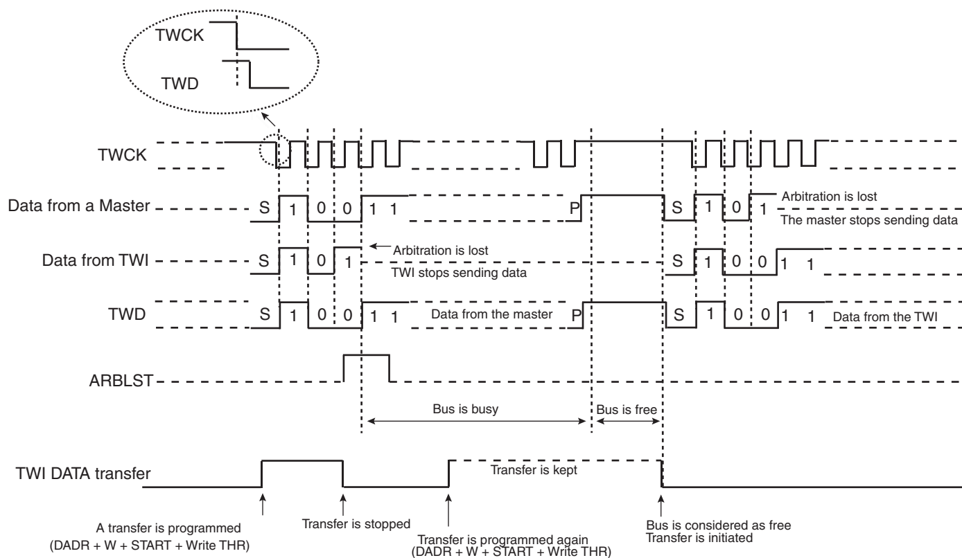
Figure 32-22. Arbitration Cases
