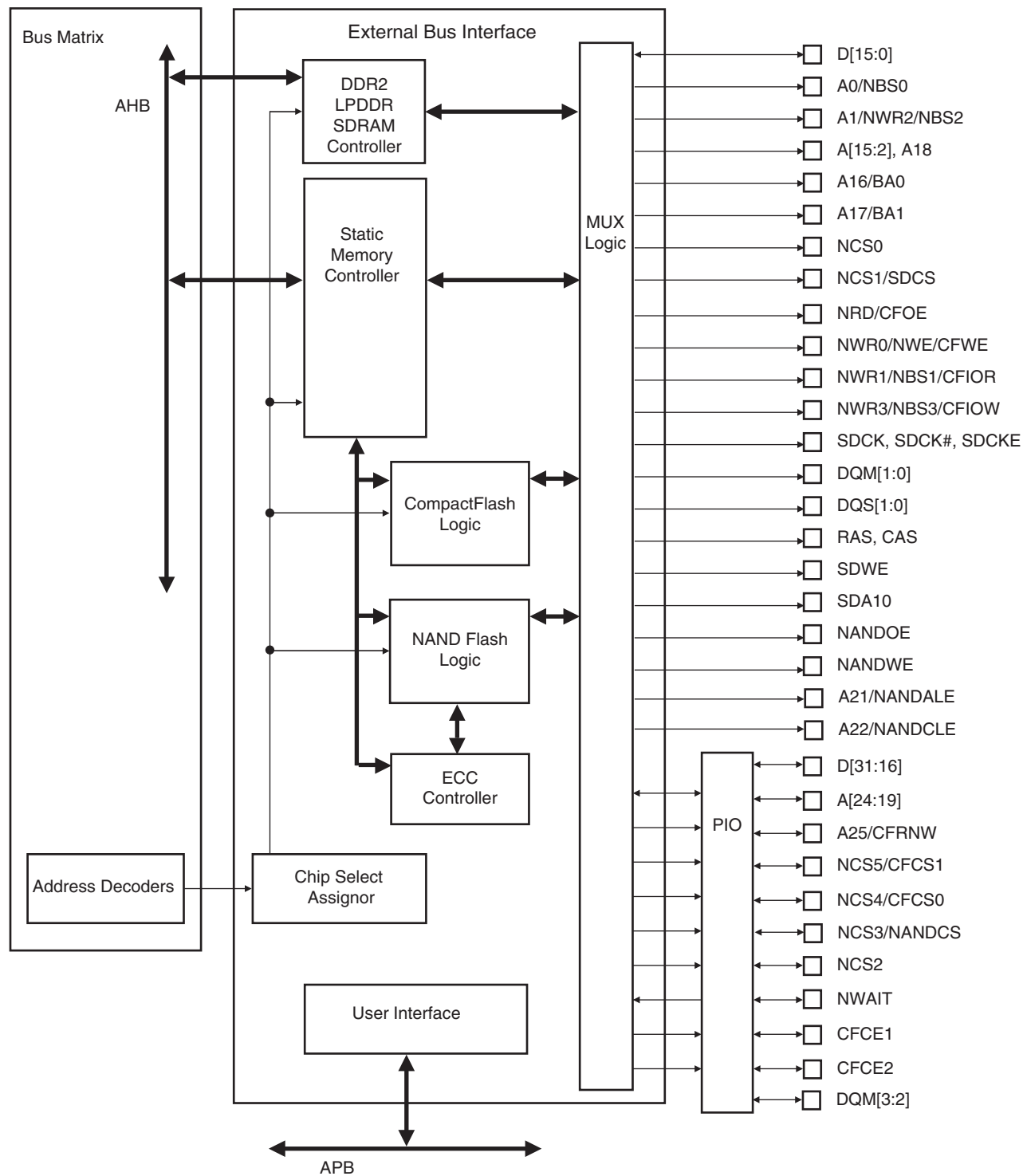
Figure 20-3. Organization of the External Bus Interface
