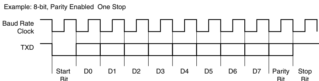
Figure 31-6. Character Transmit
