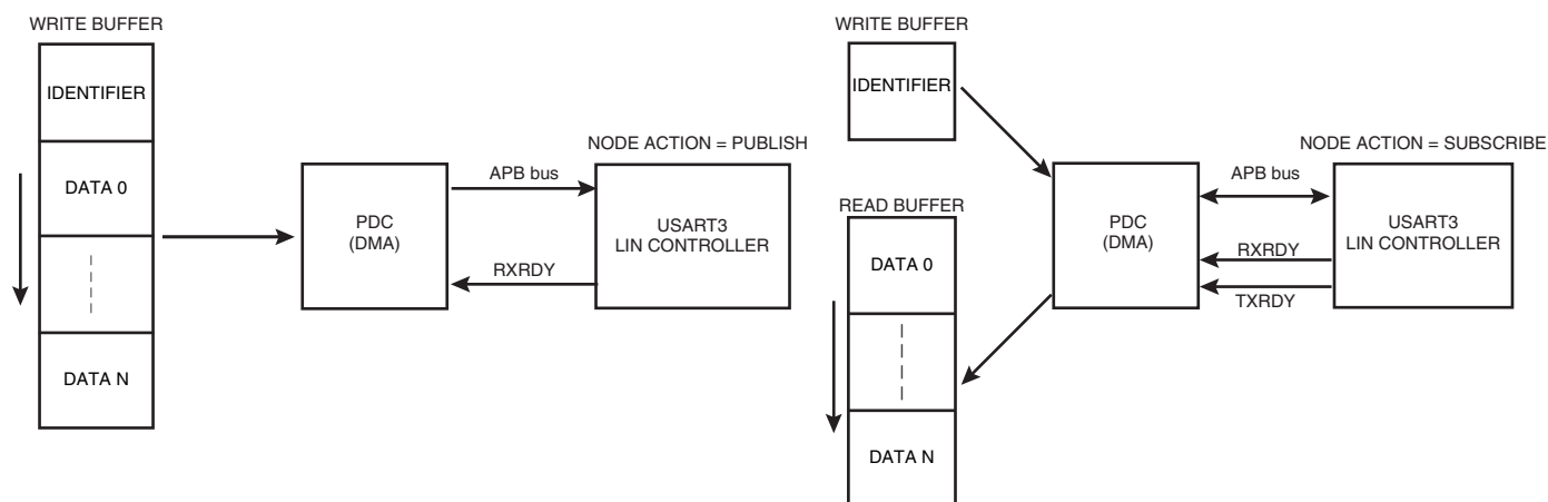
Figure 31-53. Master Node with PDC (PDCM=0)
