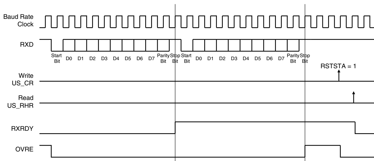
Figure 31-21. Receiver Status
