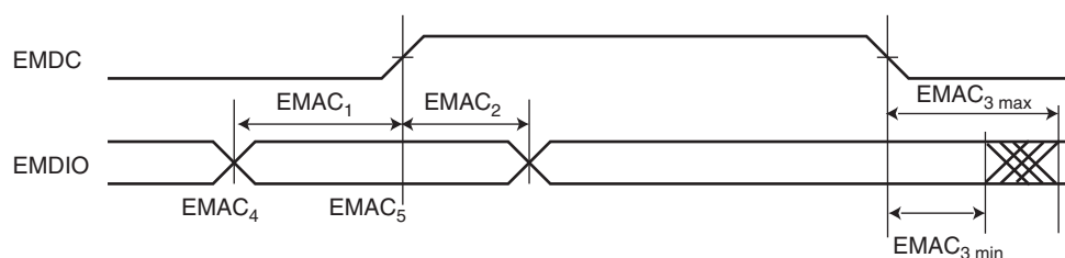
Figure 47-20. Min and Max Access Time of EMAC Output Signals
