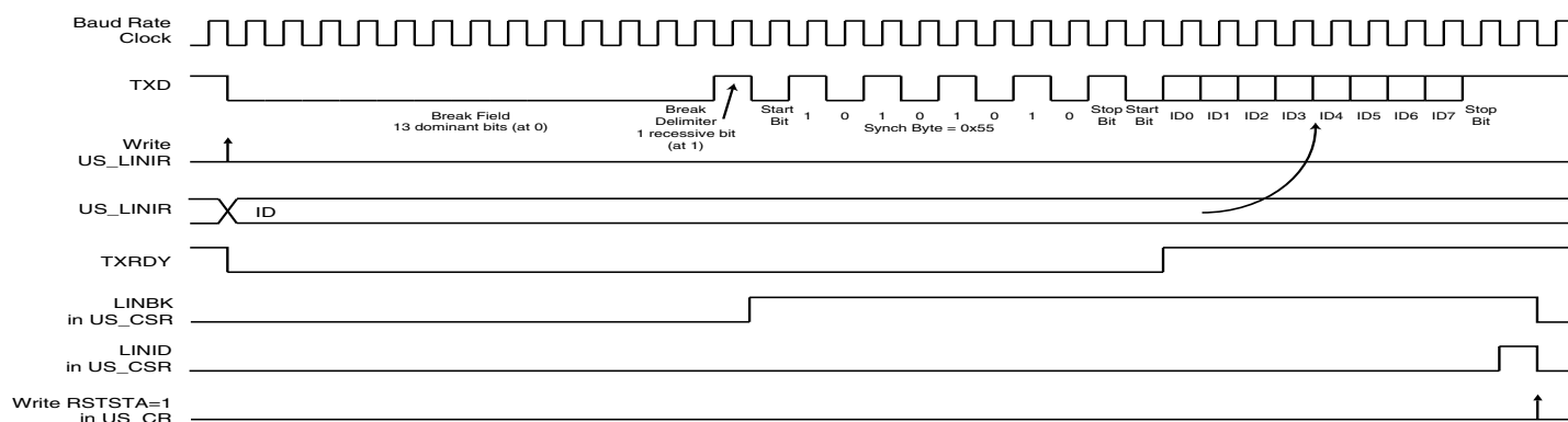
Figure 31-40. Header Transmission
