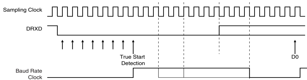
Figure 29-4. Start Bit Detection
