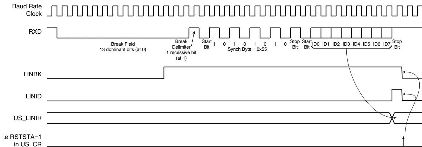
Figure 31-41. Header Reception
