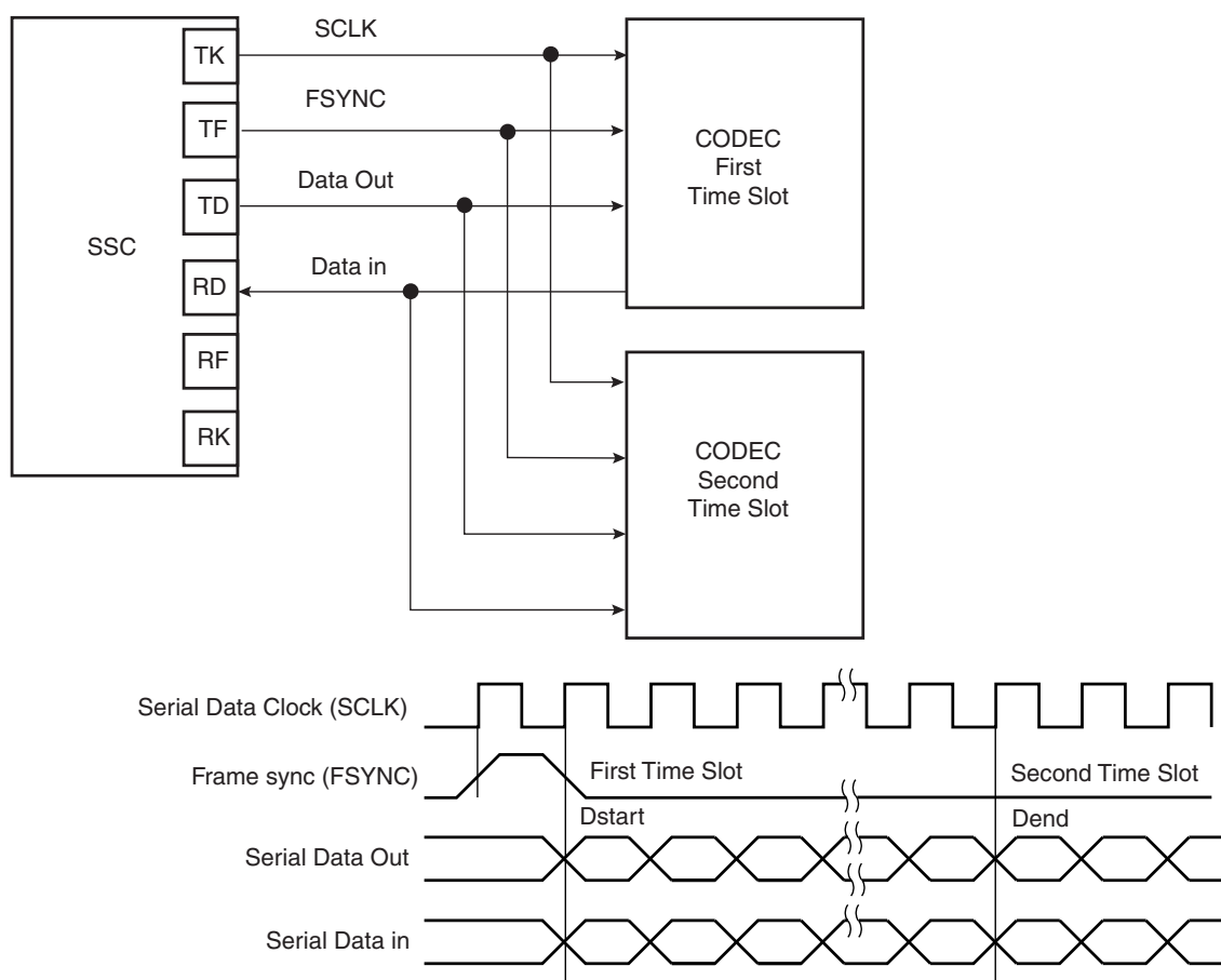
Figure 33-21. Time Slot Application Block Diagram
