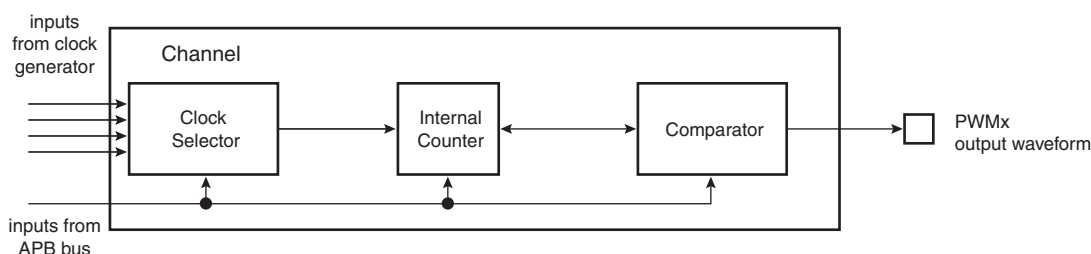
Figure 42-3. Functional View of the Channel Block Diagram
