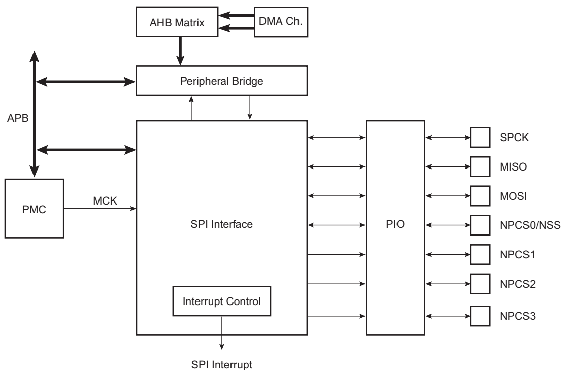
Figure 28-2. Block Diagram
