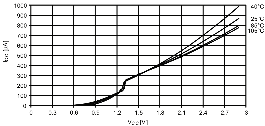
Figure 37-316. Power-on reset current consumption vs. V_{CC} .
