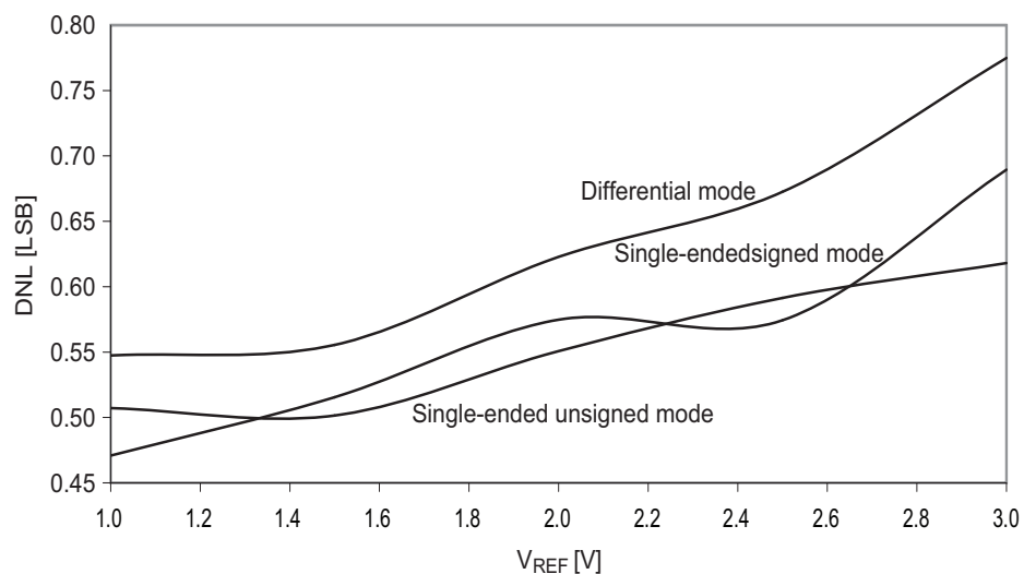
Figure 37-287. DNL error vs. external V_{REF} . T = 25^{\circ}\text{C} , V_{CC} = 3.6\text{V} , external reference.
