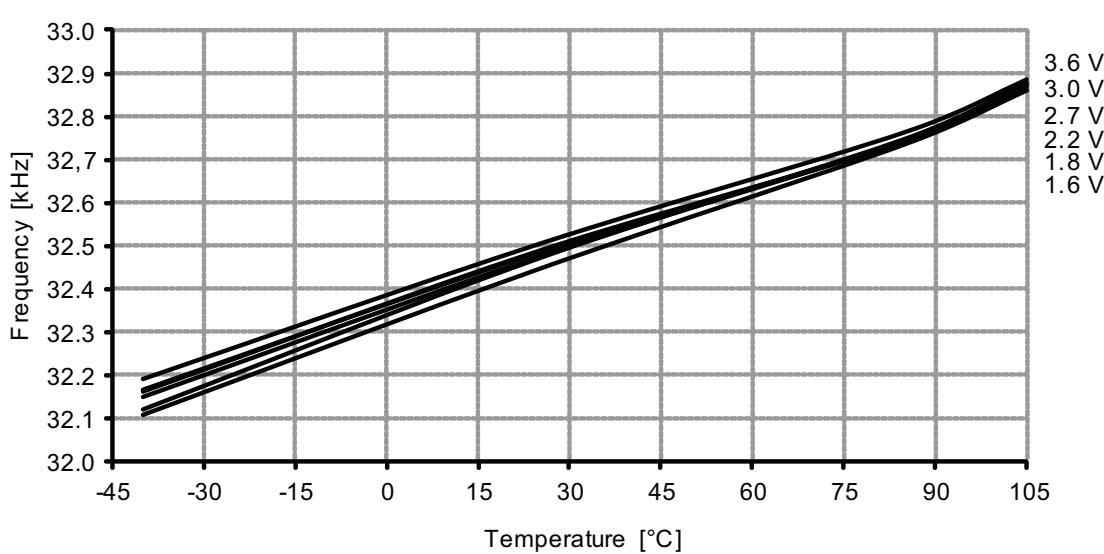
Figure 37-69. 32.768kHz internal oscillator frequency vs. temperature.
