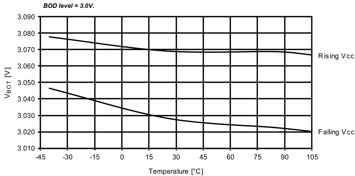
Figure 37-143. BOD thresholds vs. temperature.
