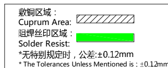
推荐焊盘尺寸 Recommended Soldering Pad
