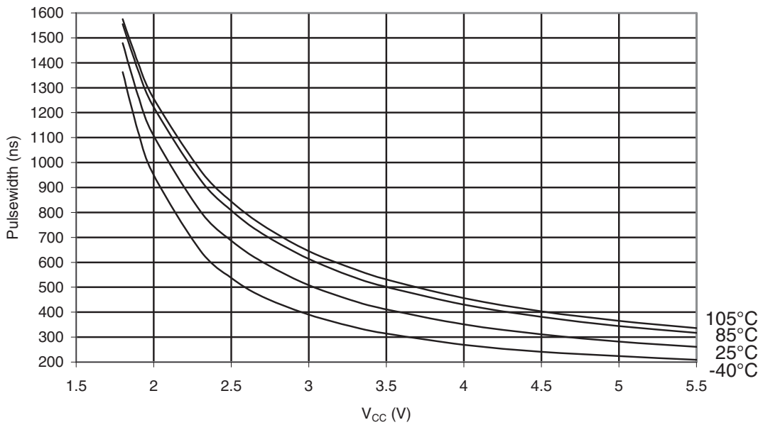
Figure 32-45. ATmega48PA: Minimum Reset Pulse width vs. V CC
