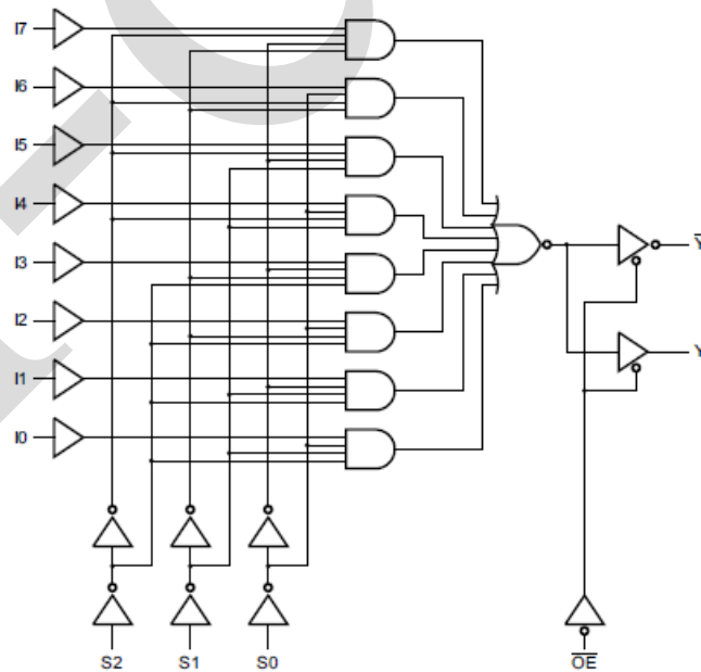
Figure 3. Logic diagram
