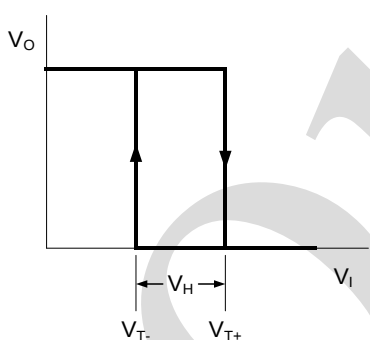
Figure 6. Transfer characteristics
