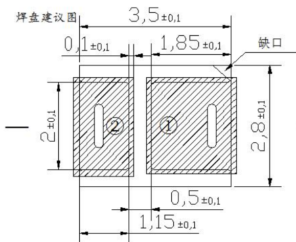
焊盘建议大小 Recommended size of pad
