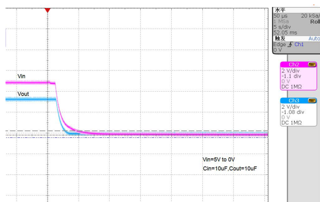
Power OFF
