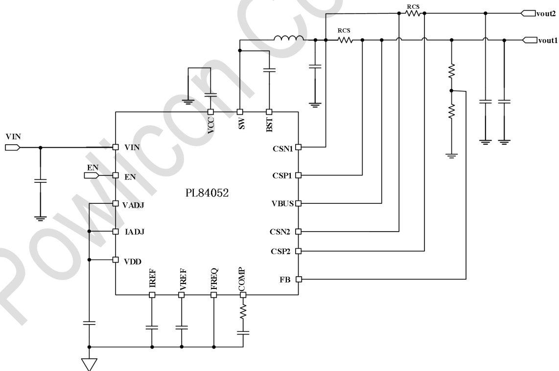
Fig. 1 Application Schematic
