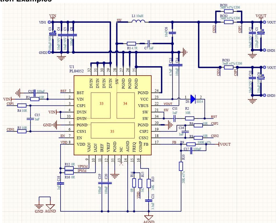
Fig. 4 Application Schematic
