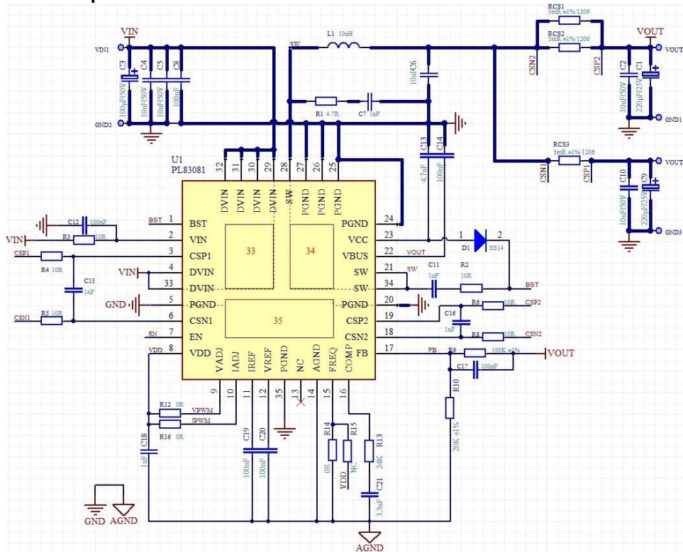
Fig. 3 Application Schematic
