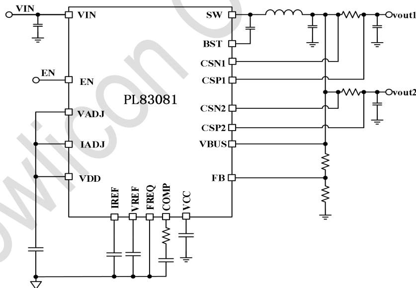
Fig. 1 Application Schematic
