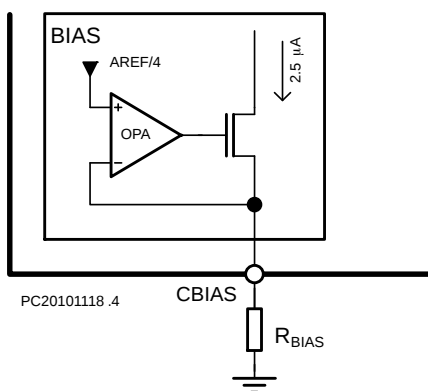
Figure 10. Bias Circuit
