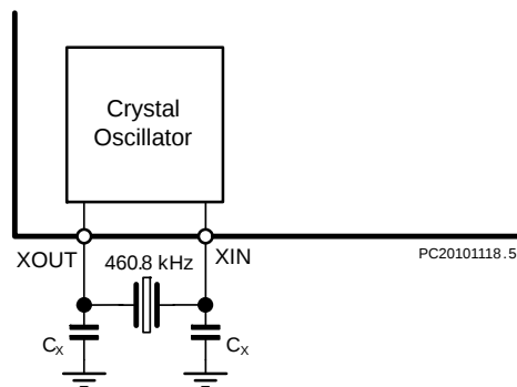
Figure 11. Crystal Oscillator
