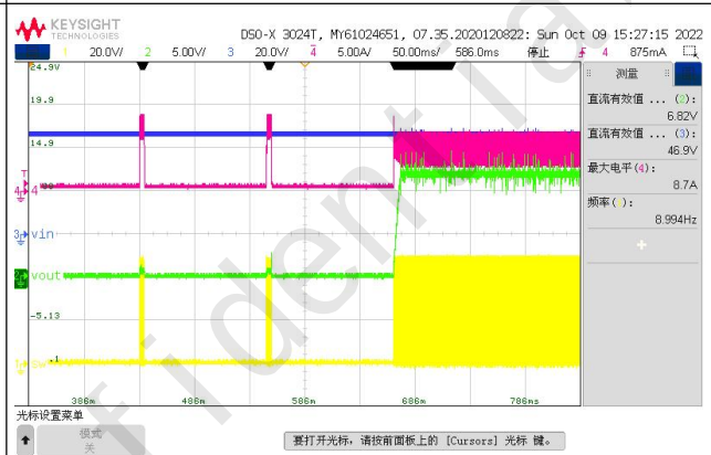
Fig. 19 Over Current Recovery
