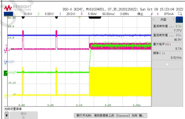
Fig. 21 Short Current Recovery
