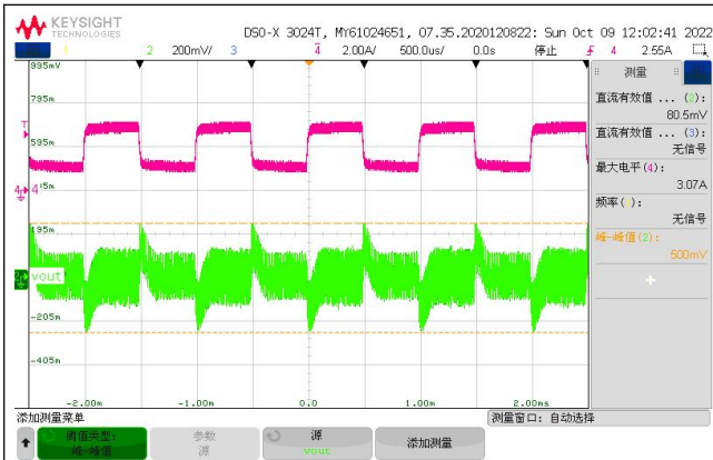
Fig. 16 Load Transient IOUT=1-3A I-ramp=1A/us
