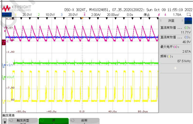
Fig. 13 Steady state DCM IOUT=1A
