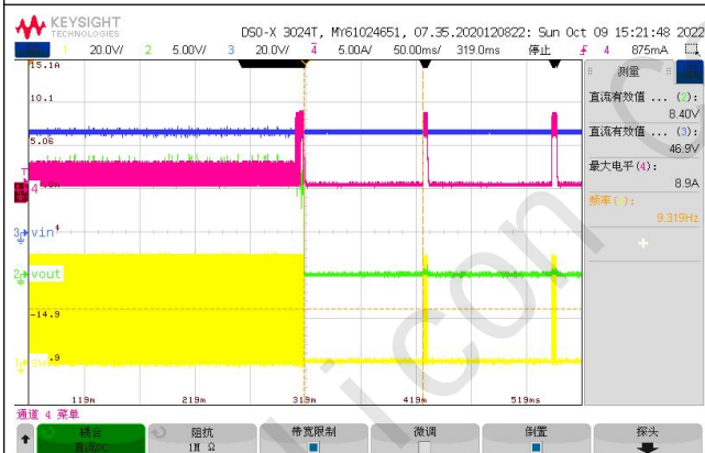
Fig. 20 Short Current Entry
