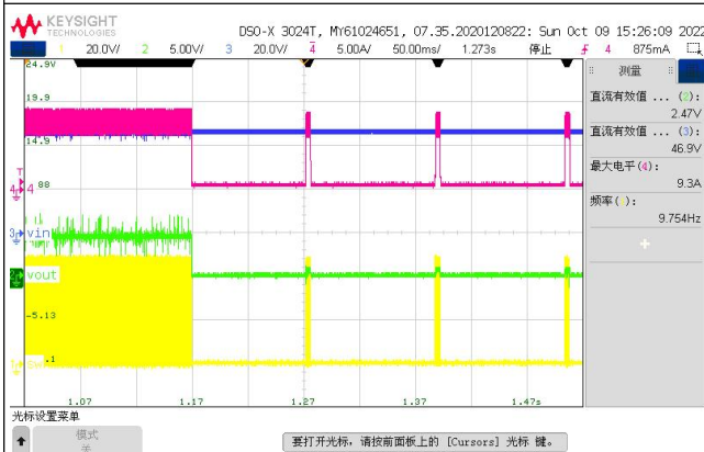
Fig. 18 Over Current Entry
