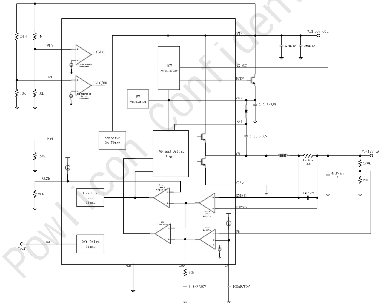
Fig. 22 Functional Block Diagram
