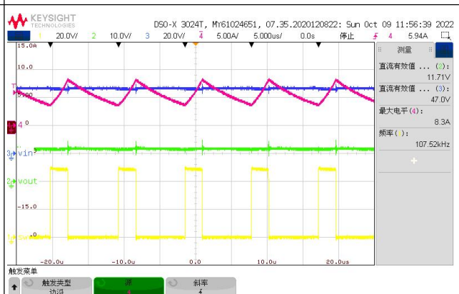
Fig. 15 Steady state CCM IOUT=5A
