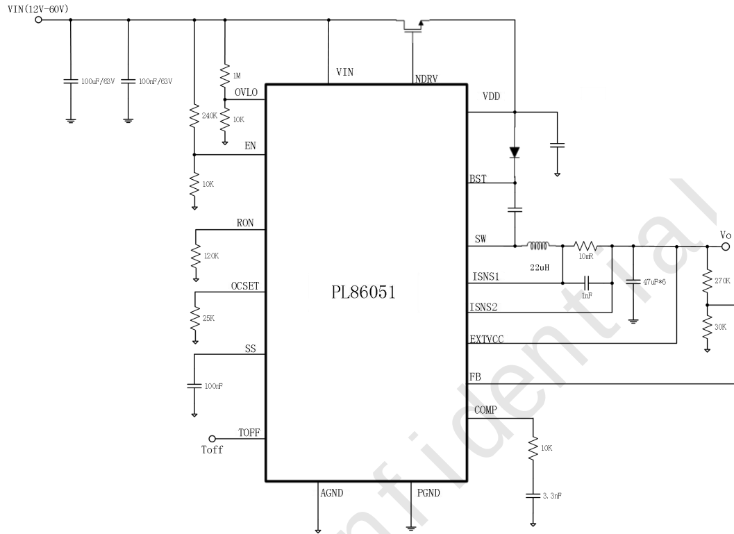
Figure 23. Application Schematic
