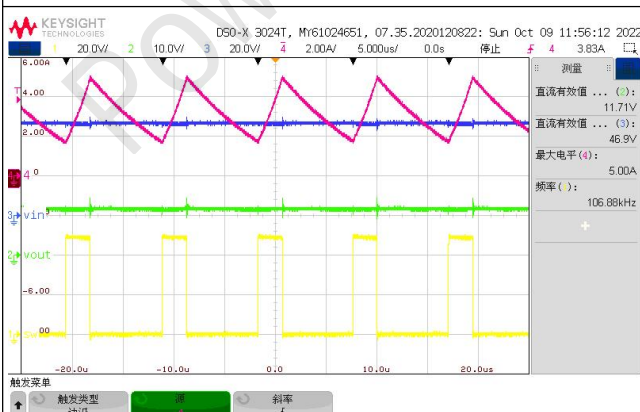
Fig. 14 Steady state CCM IOUT=3A
