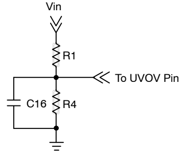
Figure 20. UV OV Bias Circuit
