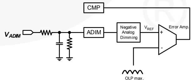
Figure 38. Analog Implementation Circuit
