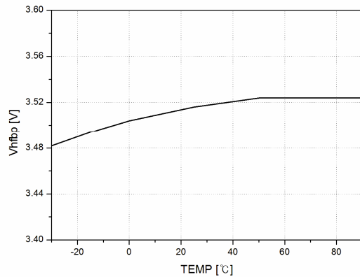
Figure 26. High-FB Protection Voltage vs. Temperature
