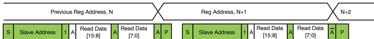
Figure 16. Single Read from Current Location
