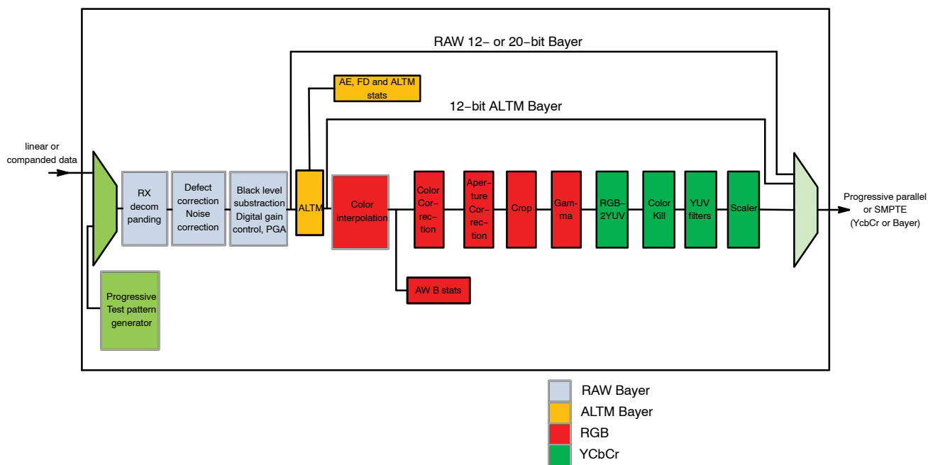
Figure 9. Continuous Mode
