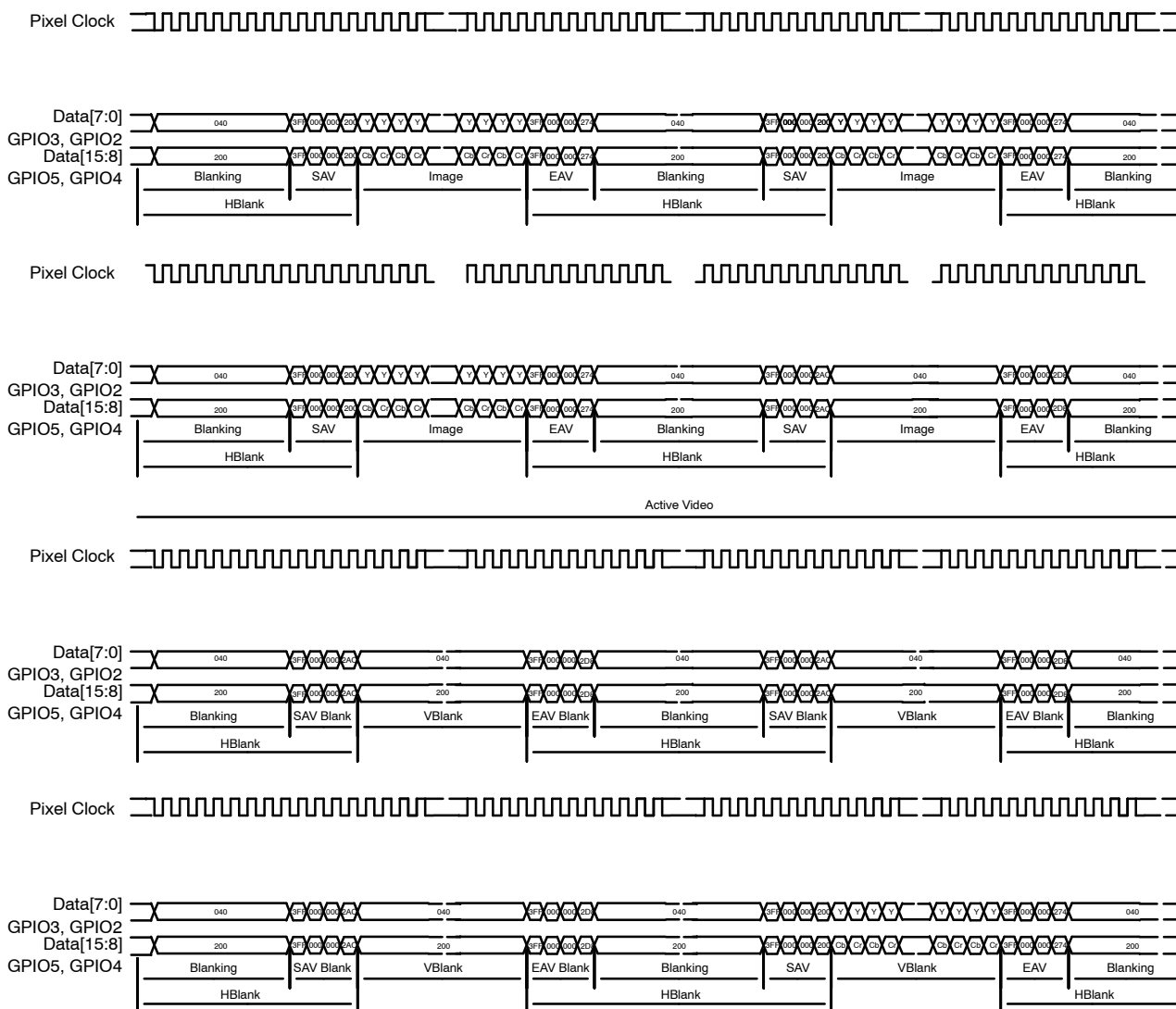
Figure 14. SMPTE296M Output
