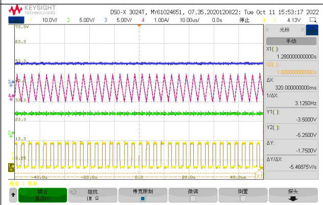
Fig.23 VIN Shut down waveform, Iout =1A
