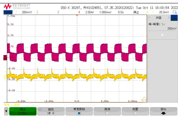
Fig.27 Steady State CCM, Iout=5A
