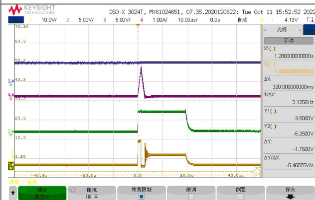
Fig.22 VIN Shut down waveform, Iout =0A
