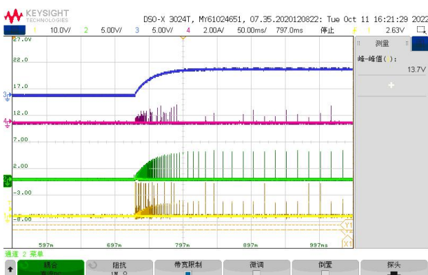
Fig.10 VIN Start up waveform, Iout =0A
