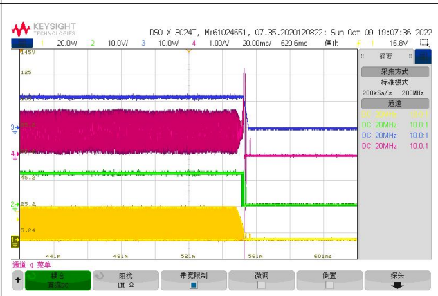
Fig.21 VIN Shut down waveform, Iout =1A
