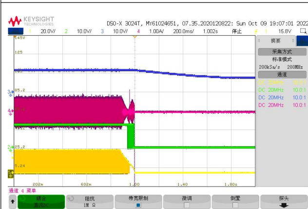
Fig.20 VIN Shut down waveform, Iout =0A
