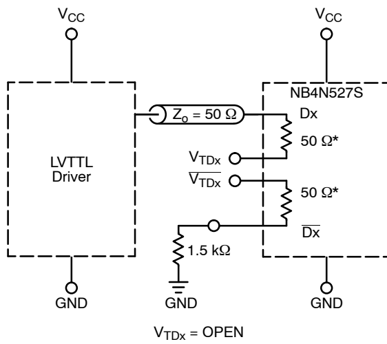
Figure 12. LVTTTL Interface
