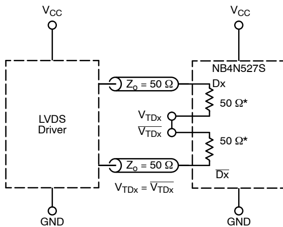
Figure 8. LVDS Interface
