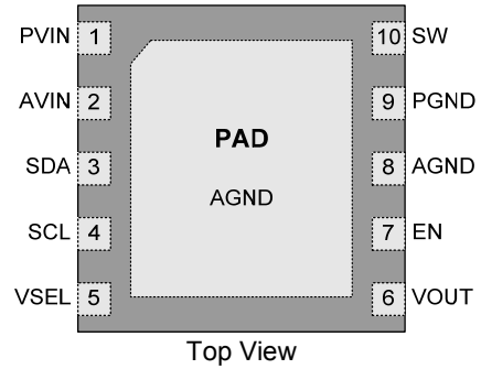
Figure 3. MLP10, 3x3mm
