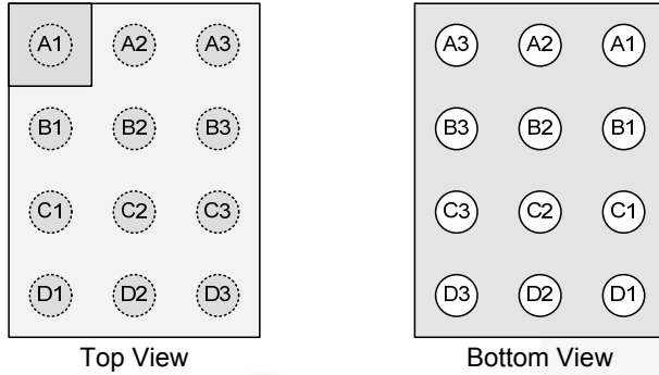
Figure 2. WLCSP-12, 2.23x1.46mm
