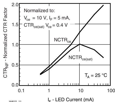
Fig. 11 - Normalization Factor for Non-Saturated and Saturated CTR vs. I_F
