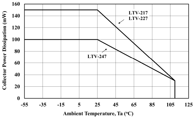
Figure 1. Collector Power Dissipation vs. Ambient Temperature
