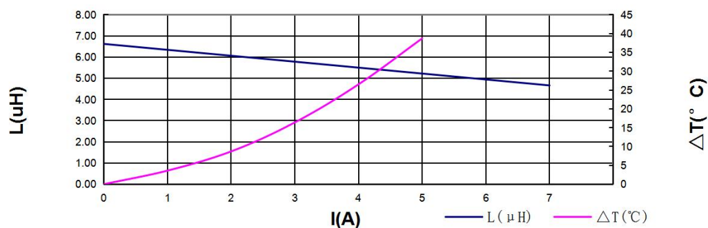
CURRENT CHARACTERISTIC
