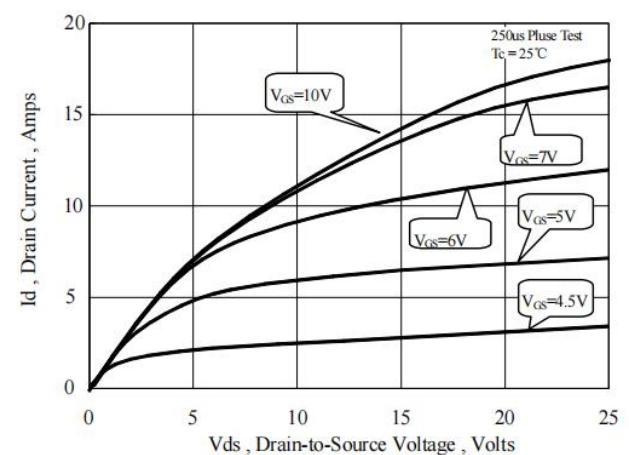
Figure 6. On-State Characteristics
