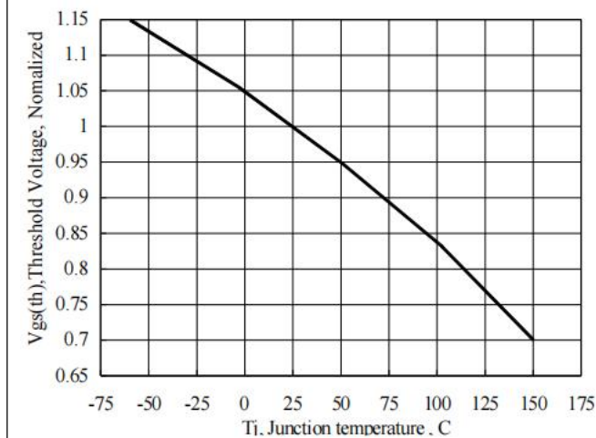
Figure 3. Gate Threshold Variation with Temperature
