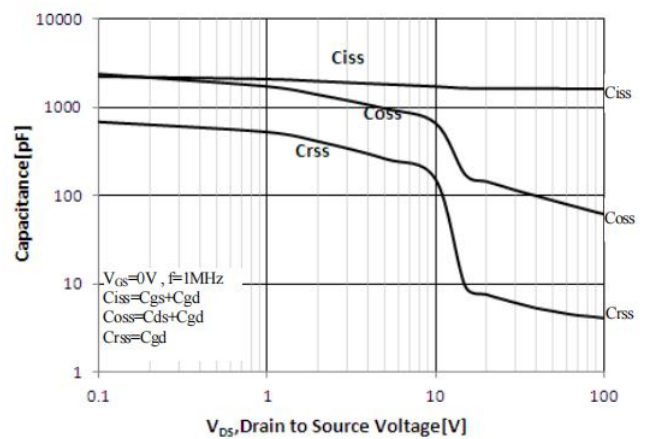
Figure 4. Capacitance Characteristics
