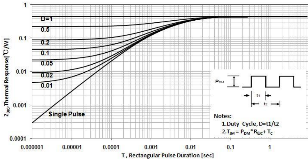
Figure 9. Maximum Effective Thermal Impedance , Junction to Case
